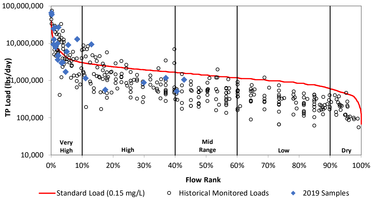
Figure 25g. Load duration curve for total phosphorus at SB802.
