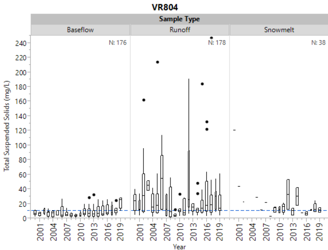
Figure 20c. Historical total suspended solids by sample type at VR804.
