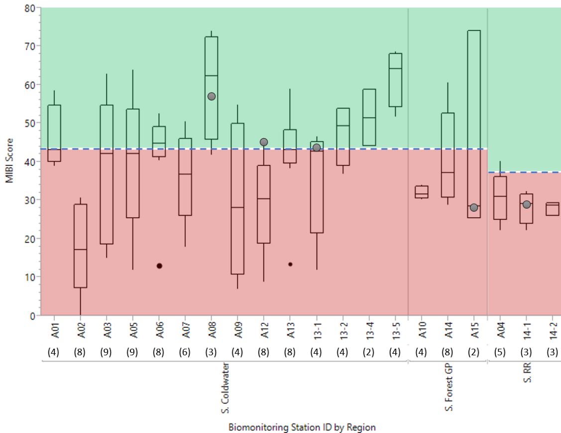
Figure 29. Macroinvertebrate Index of Biological Integrity (MIBI) score by region. Number of samples collected from 2009-2019 is shown in parenthesis (see Appendix for more details). The impairment threshold is indicated by a dashed blue line. Sites with scores above the threshold value (green area), are likely not to be considered 'impaired'. Sites with scores below the threshold value (red area), are likely to be considered 'impaired'. Sites monitored in 2019 have a grey circle indicating the MIBI score.
