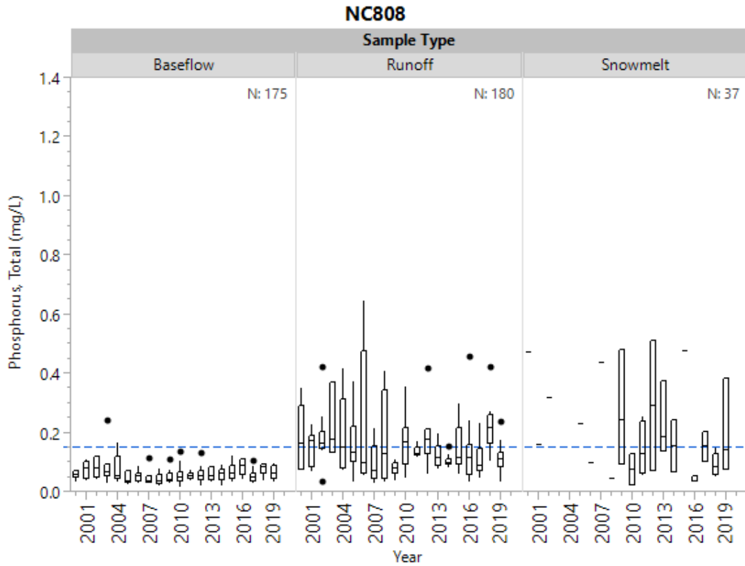
Figure 16e. Historical total phosphorus by sample type at NC808.
