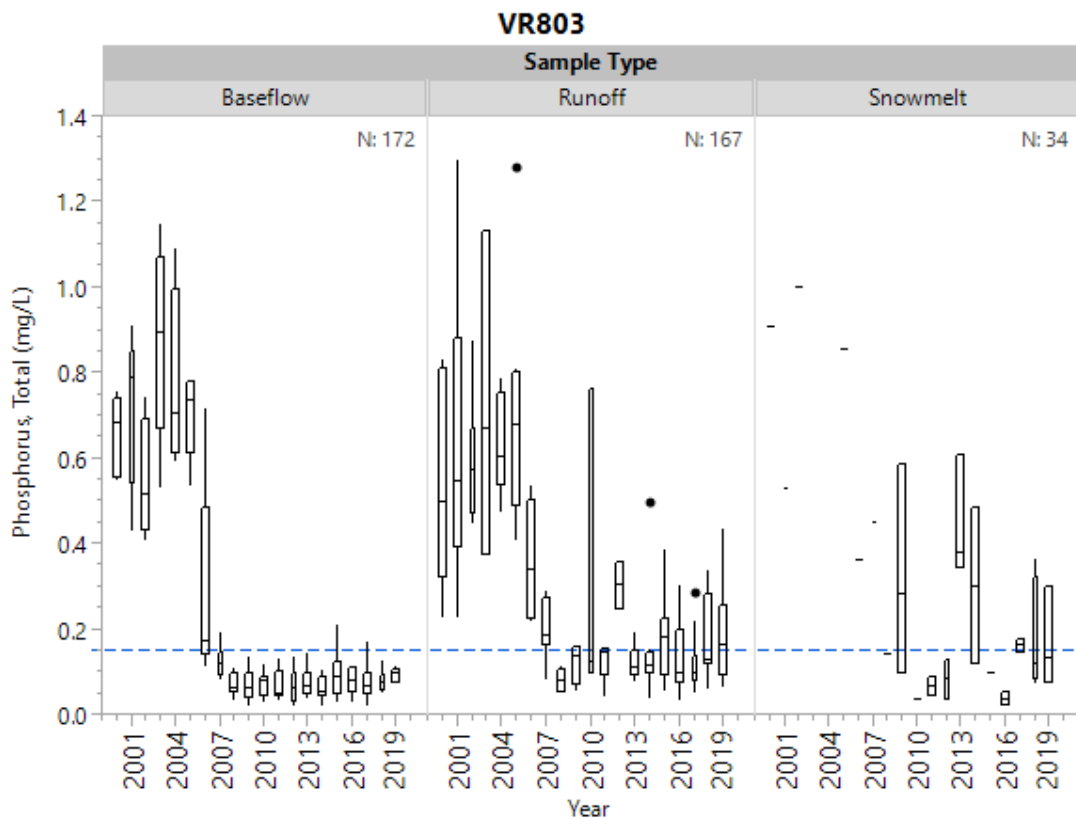
Figure 16h. Historical total phosphorus by sample type at VR803.
