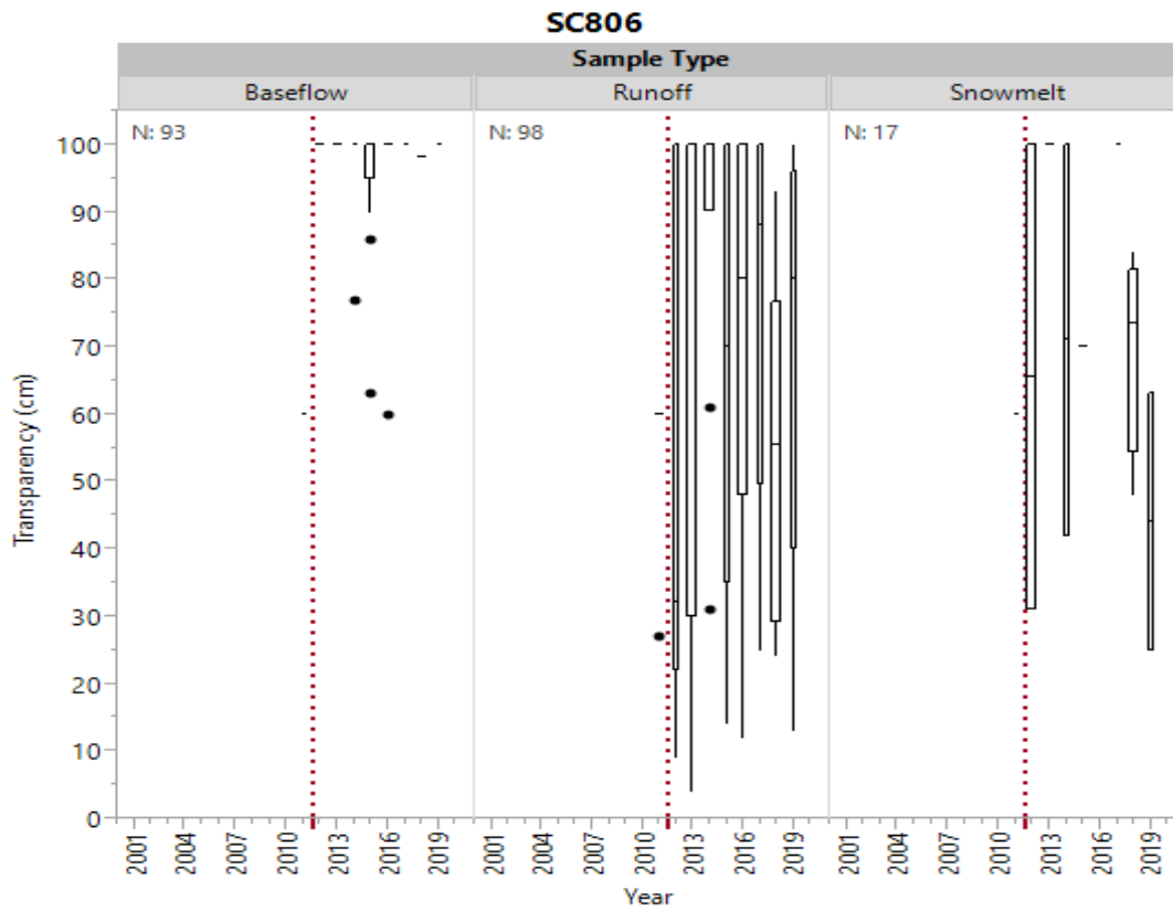
Figure 22b. Historical transparency by sample type for SC806.
