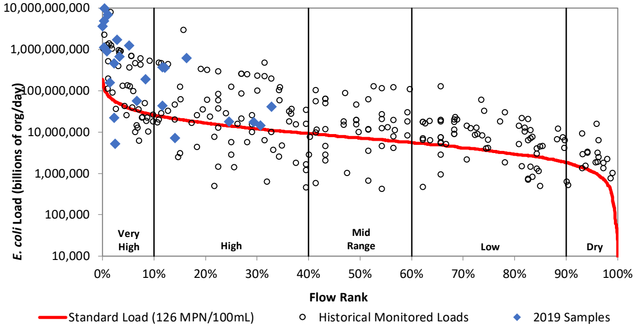
Figure 23c. Load duration curve for E. coli at VR804.
