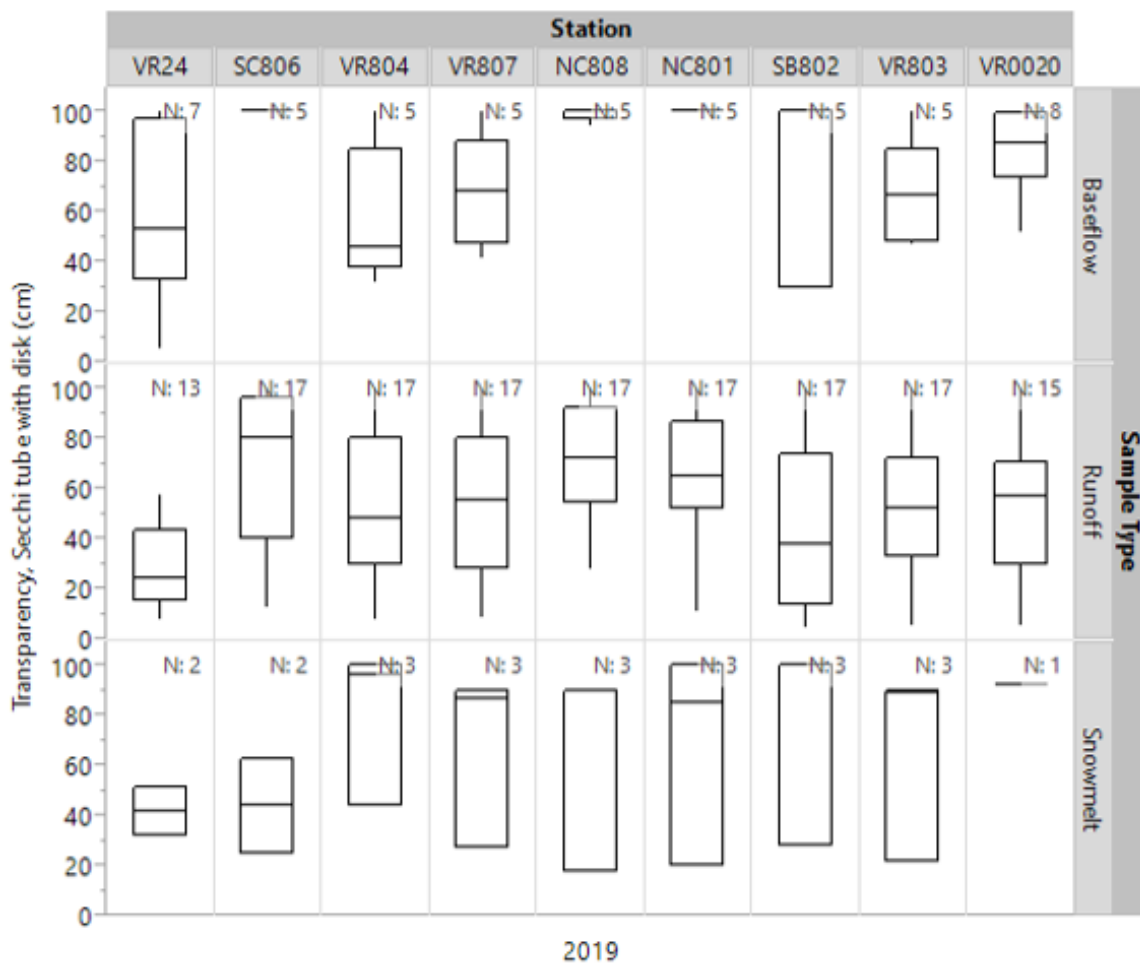
Figure 21. Transparency, categorized by sample type, for 2019.
