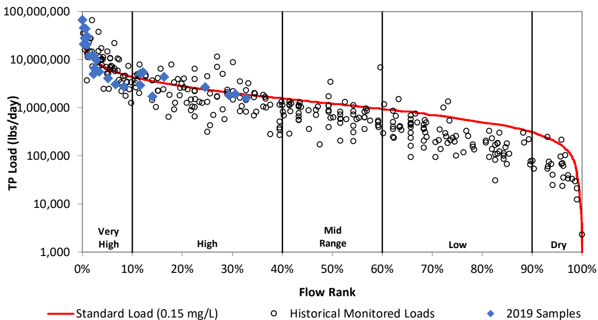
Figure 25c. Load duration curve for total phosphorus at VR804.
