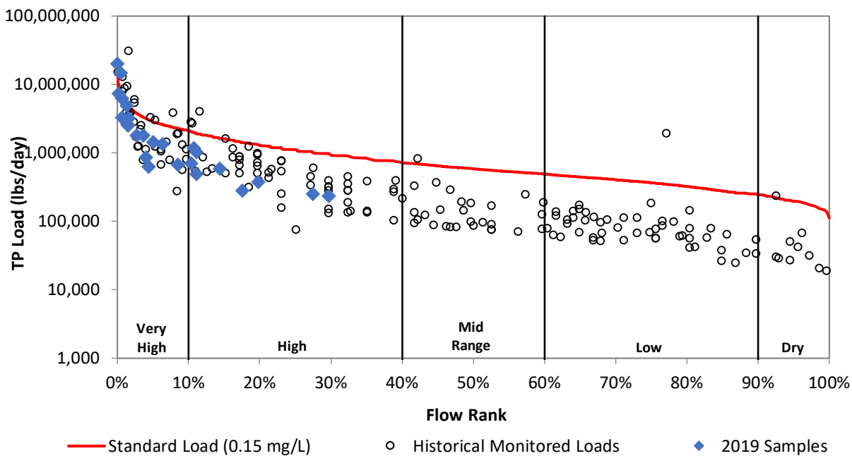
Figure 25b. Load duration curve for total phosphorus at SC806.
