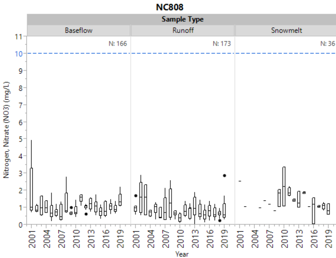
Figure 14e. Historical nitrate by sample type for NC808.
