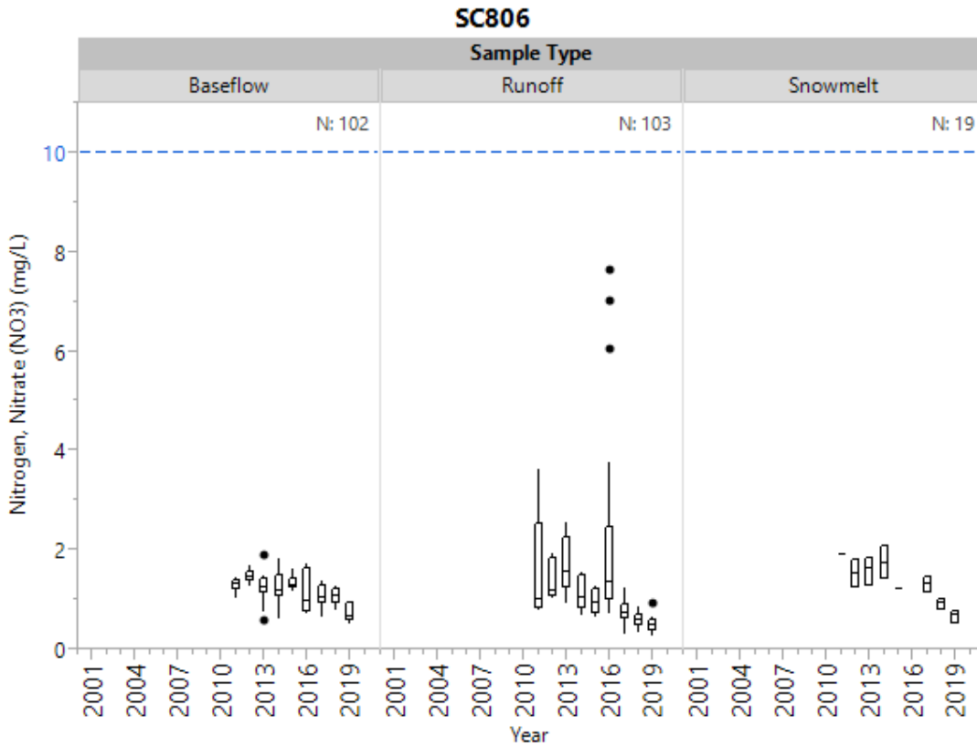
Figure 14b. Historical nitrate by sample type for SC806.
