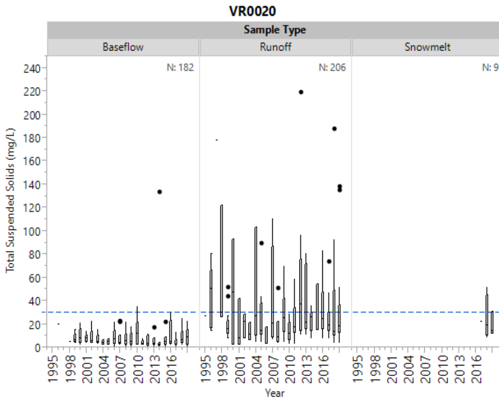
Figure 20i. Historical total suspended solids by sample type at VR0020.
