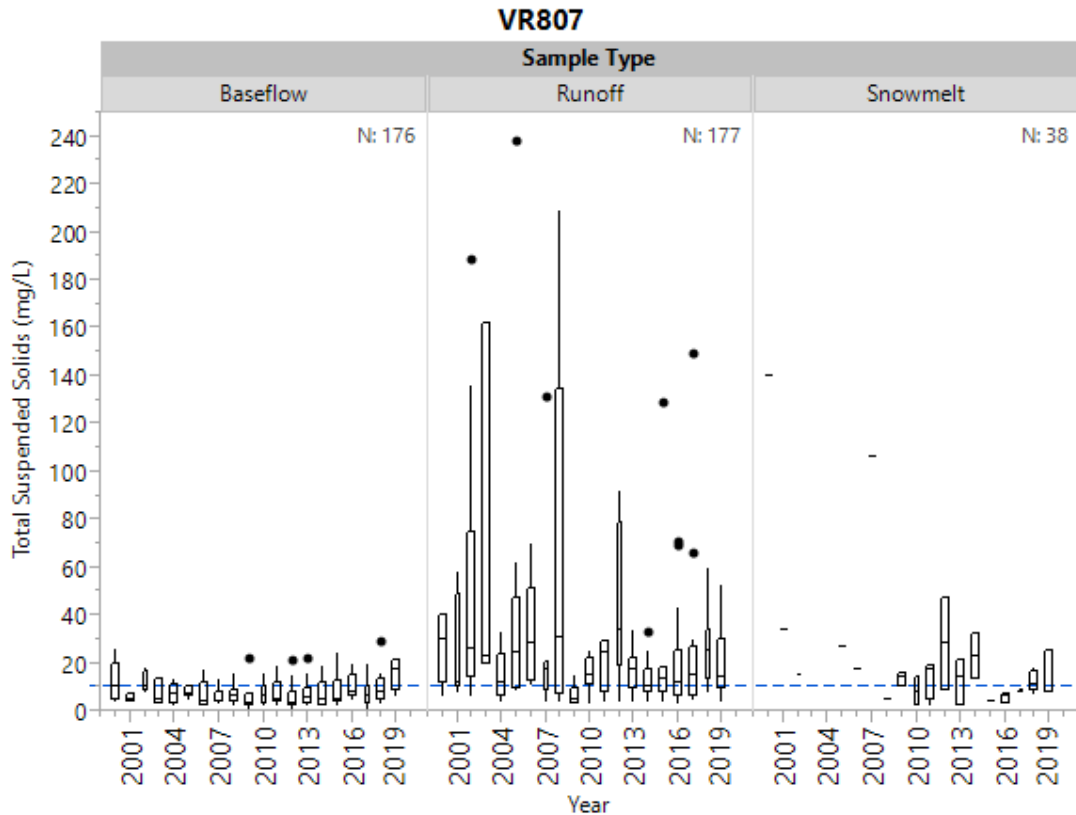
Figure 20d. Historical total suspended solids by sample type at VR807.
