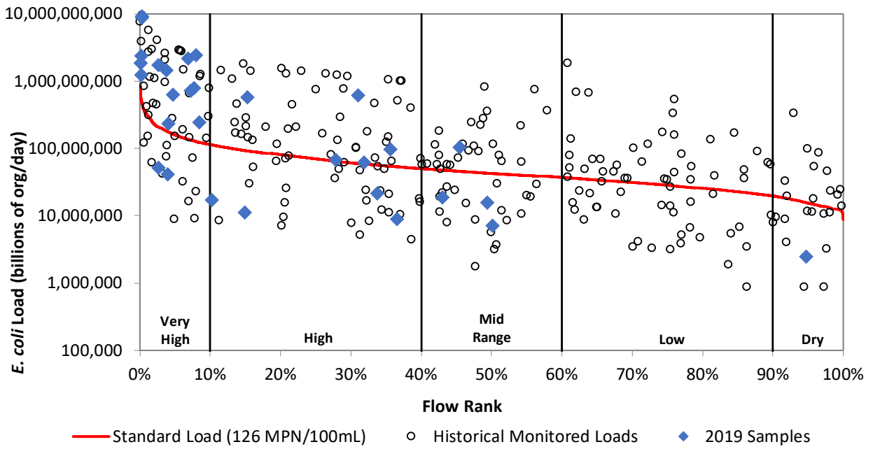
Figure 23i. Load duration curve for E. coli at VR0020.
