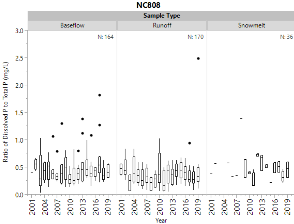
Figure 18e. Historical ratio of dissolved phosphorus to total phosphorus by sample type at NC808.
