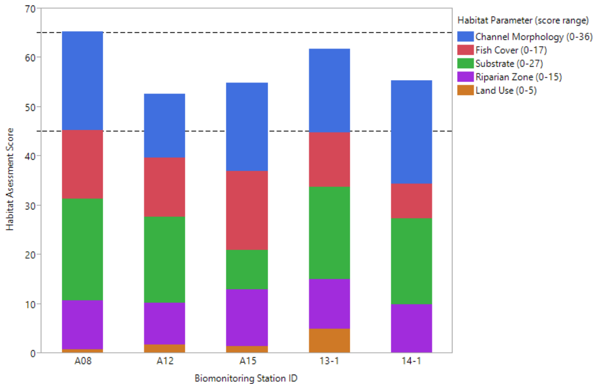
Figure 31. Habitat assessment score by habitat parameter for each biomonitoring station in 2019. Dashed black lines indicate limits for Good ( \geq 66 ), Fair (45-65), and Poor ( \leq 44 ) categories based on the total habitat assessment score (total score of 100).
