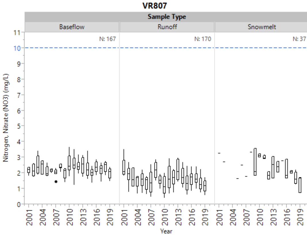
Figure 14d. Historical nitrate by sample type for VR807.
