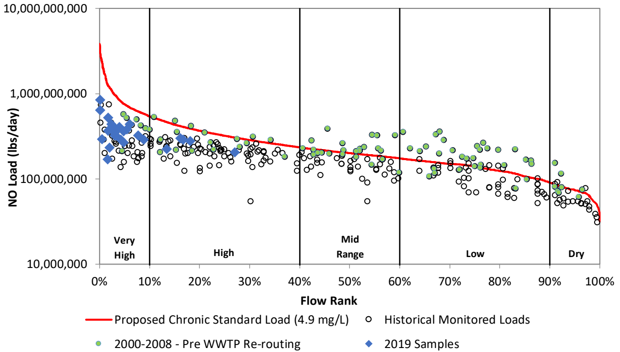
Figure 24h. Load duration curve for nitrate at VR803.
