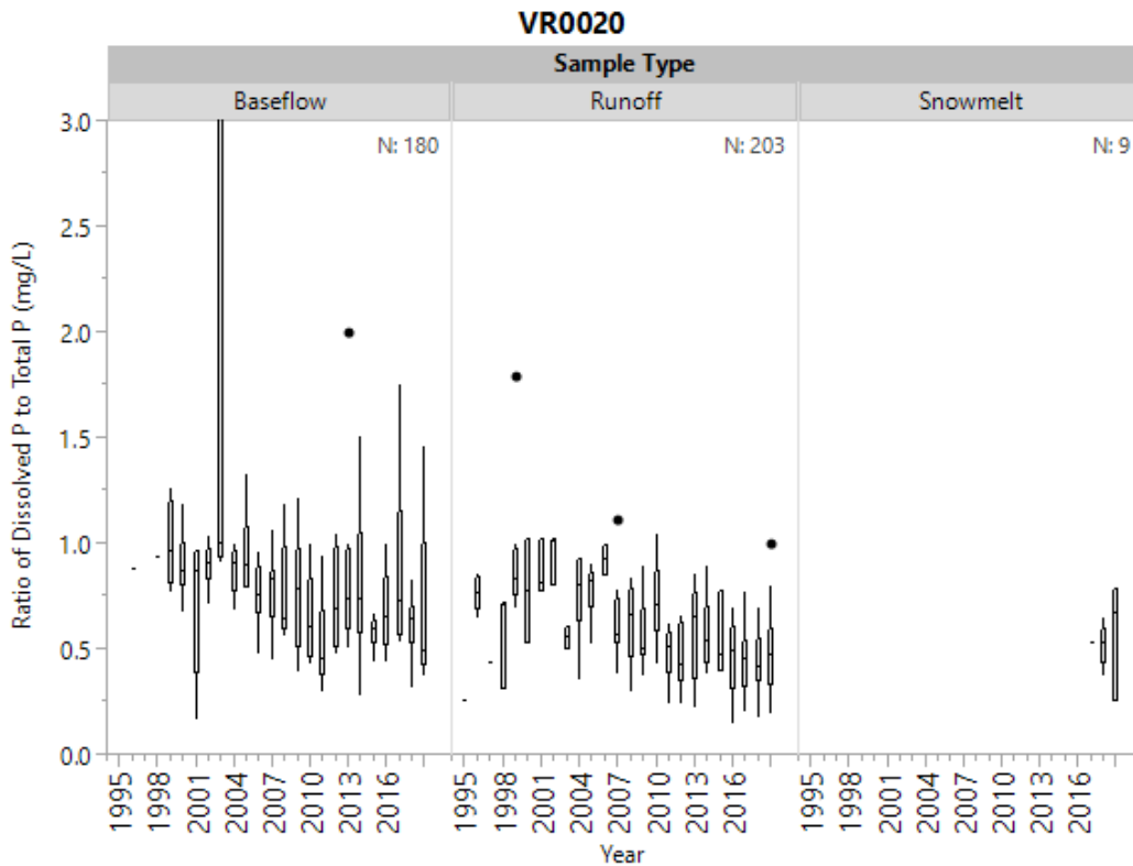
Figure 18i. Historical ratio of dissolved phosphorus to total phosphorus by sample type at VR0020.
