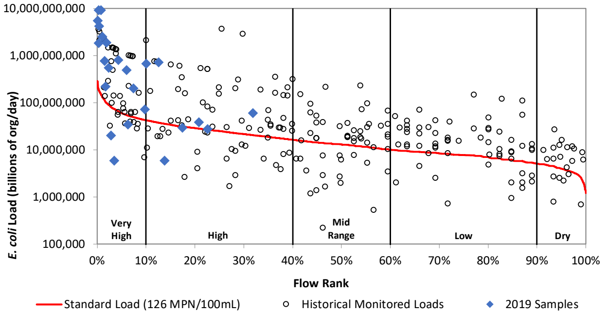
Figure 23d. Load duration curve for E. coli at VR807.
