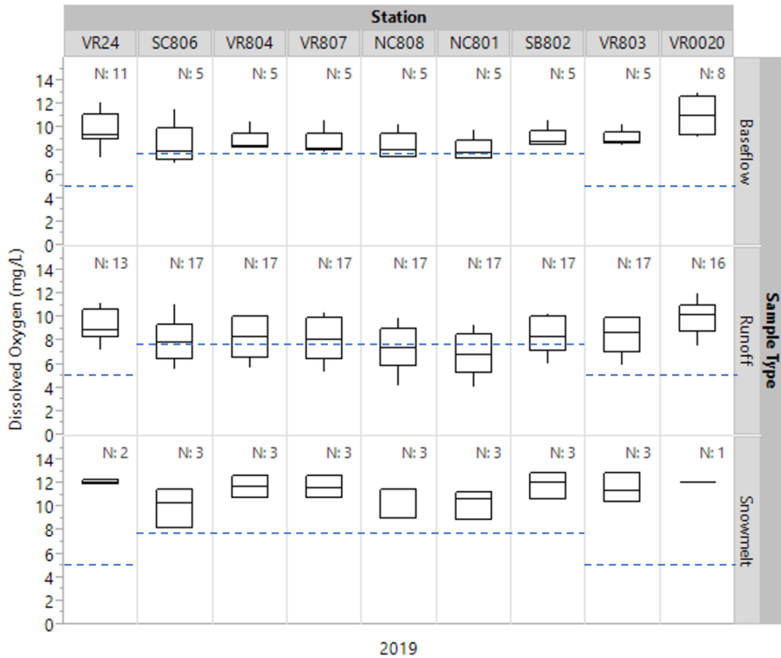
Figure 9. Dissolved oxygen for each station, categorized by sample type, for 2019.
