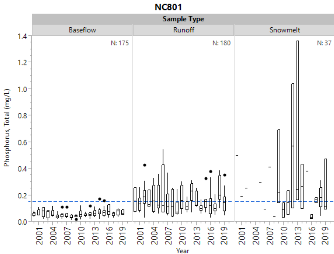
Figure 16f. Historical total phosphorus by sample type at NC801.
