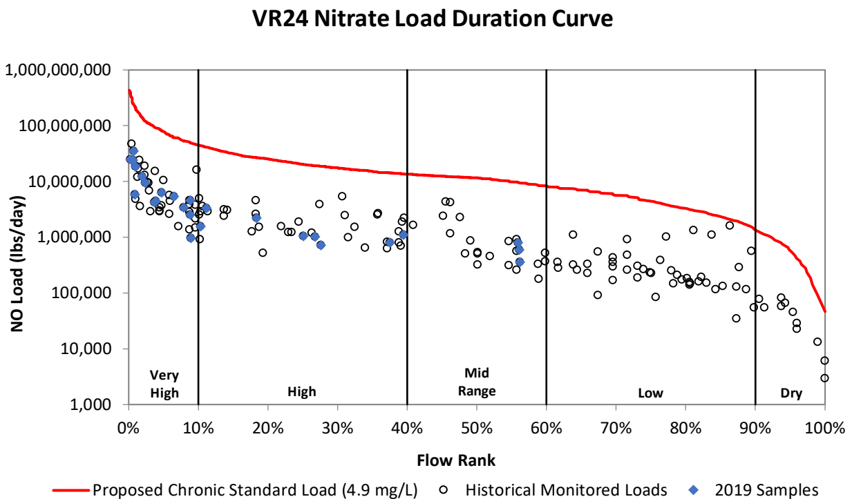
Figure 24a. Load duration curve for nitrate at VR24.
