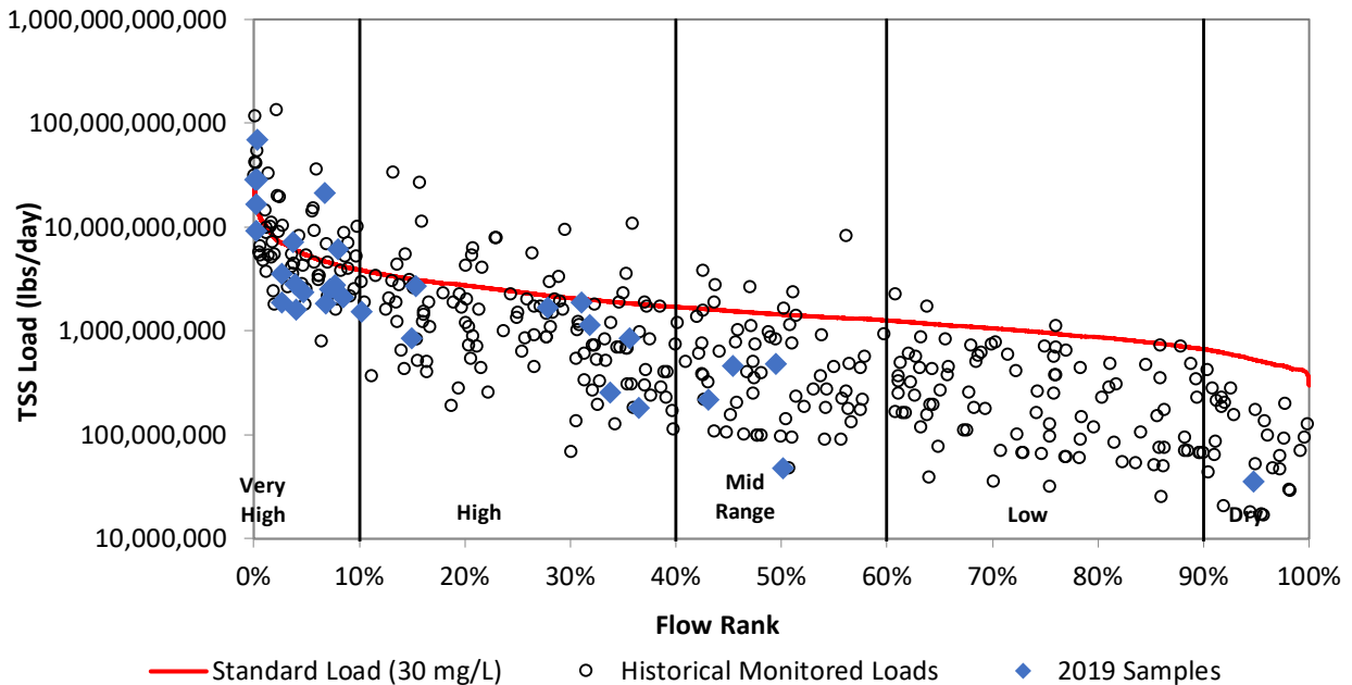
Figure 26i. Load duration curve for total suspended solids at VR0020.
