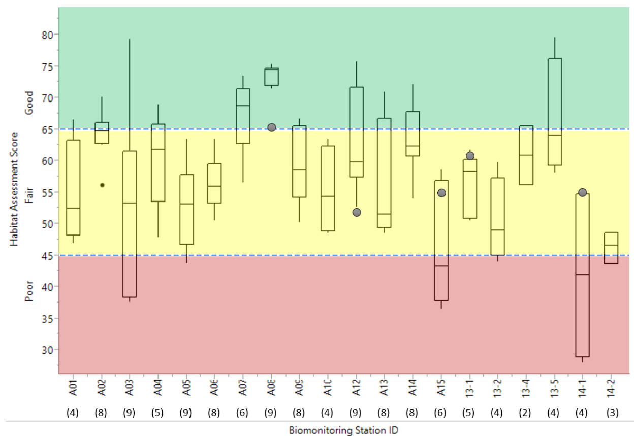
Figure 30. Habitat assessment scores for biomonitoring stations. Habitat scores for 2019 are indicated by grey circle. Dashed blue lines indicate limits for Good ( \geq 66 ), Fair (45-65), and Poor ( \leq 44 ) categories. Number of samples collected from 2009-2019 is shown in parenthesis (see Appendix for more details).
