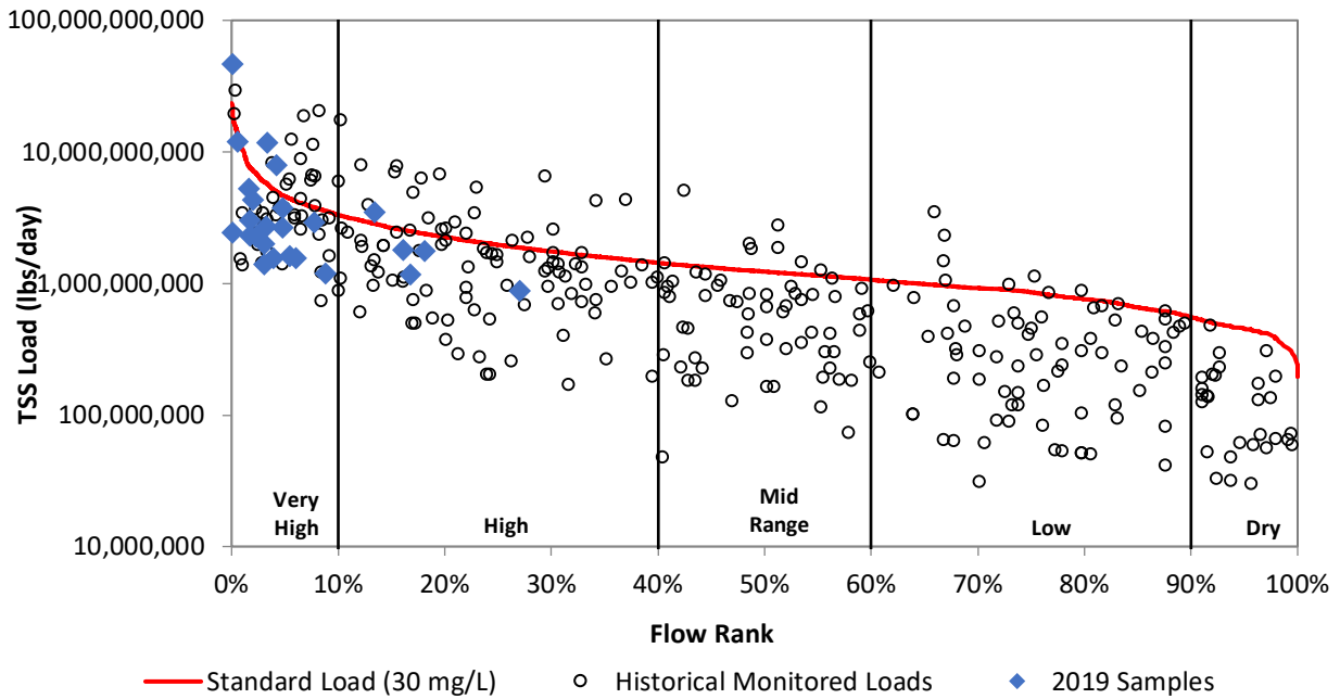
Figure 26h. Load duration curve for total suspended solids at VR803.
