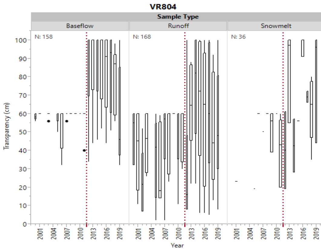
Figure 22c. Historical transparency by sample type for VR804.
