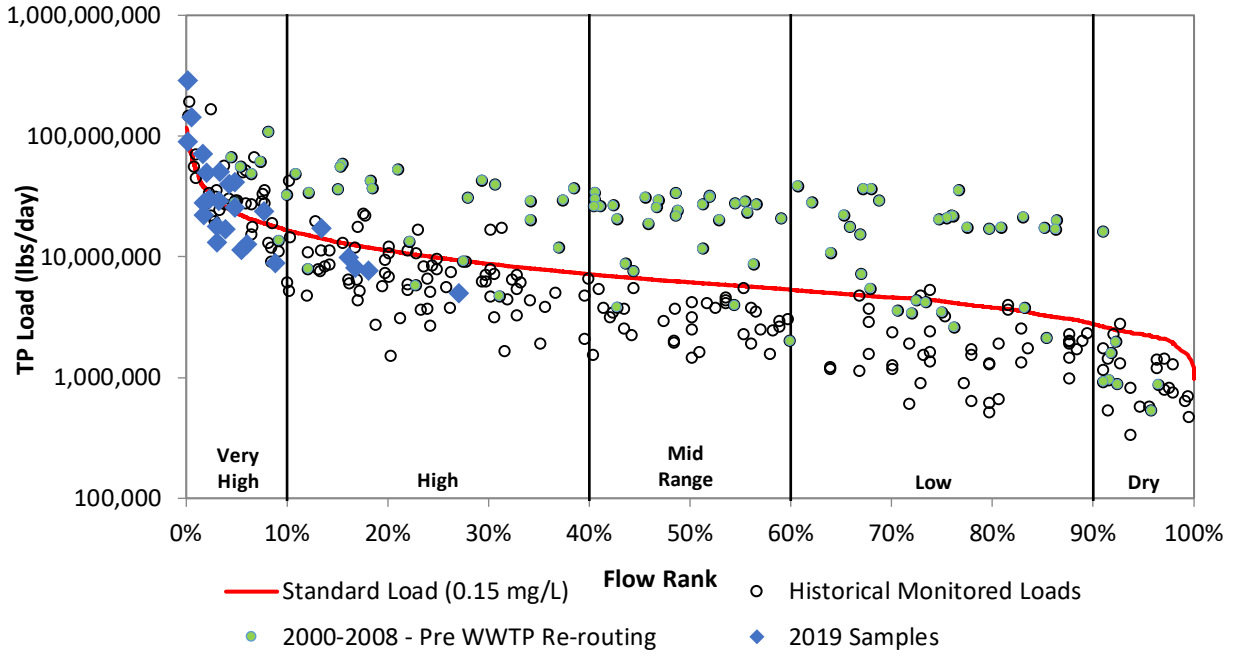
Figure 25h. Load duration curve for total phosphorus at VR803.
