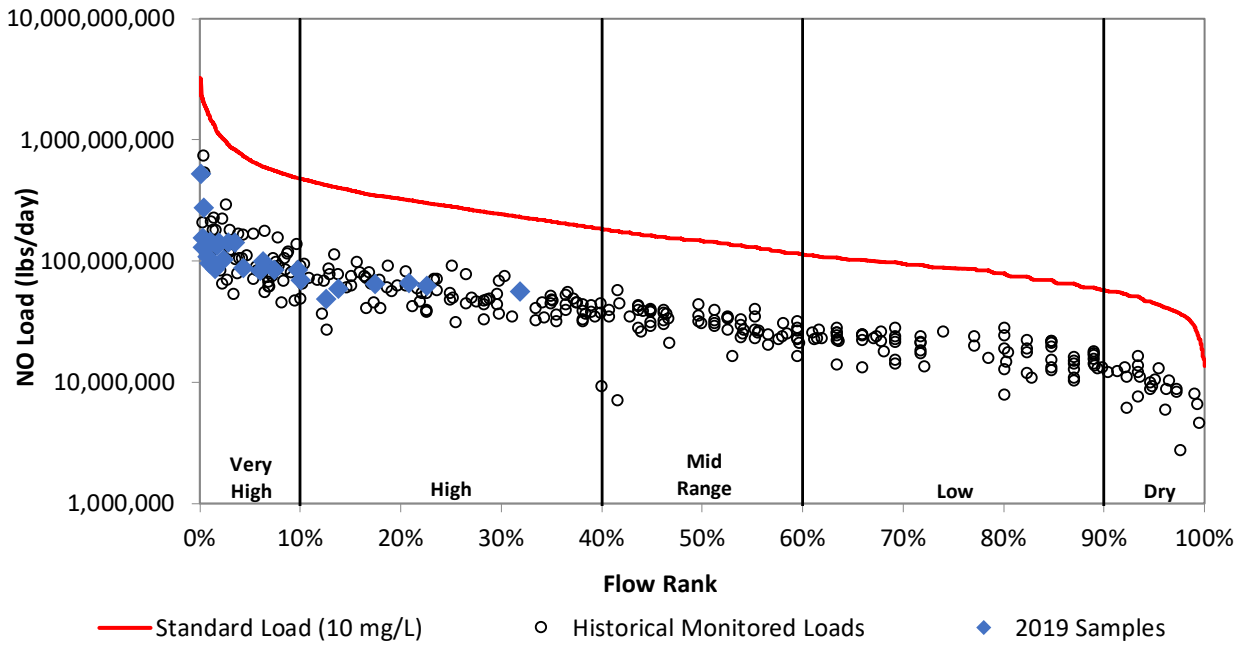
Figure 24d. Load duration curve for nitrate at VR807.
