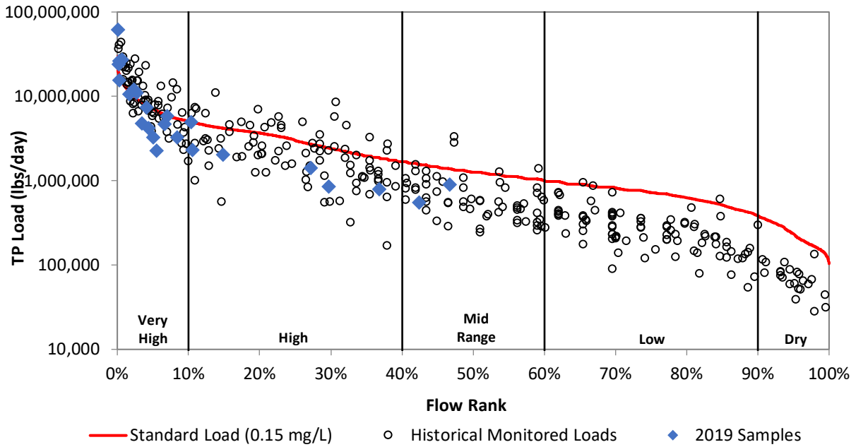
Figure 25f. Load duration curve for total phosphorus at NC801.
