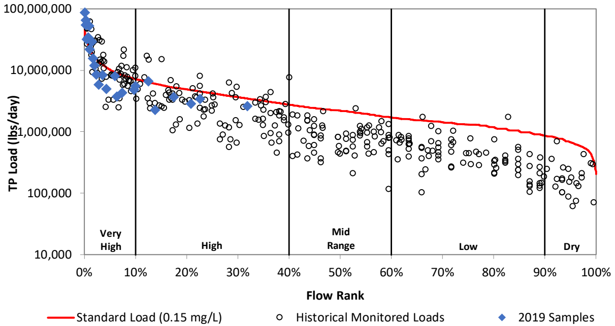
Figure 25d. Load duration curve for total phosphorus at VR807.
