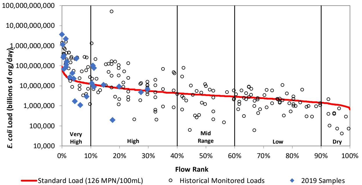
Figure 23b. Load duration curve for E. coli at SC806.
