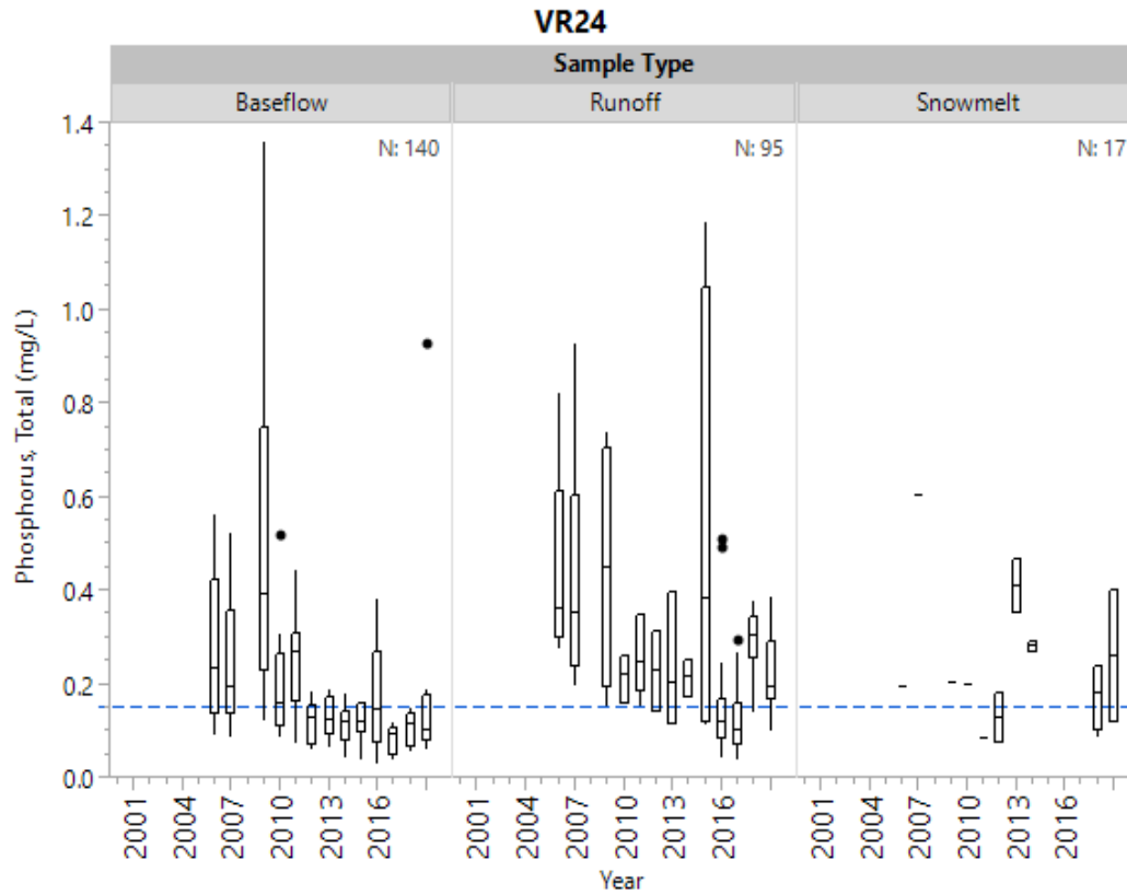
Figure 16a. Historical total phosphorus by sample type at VR24.
