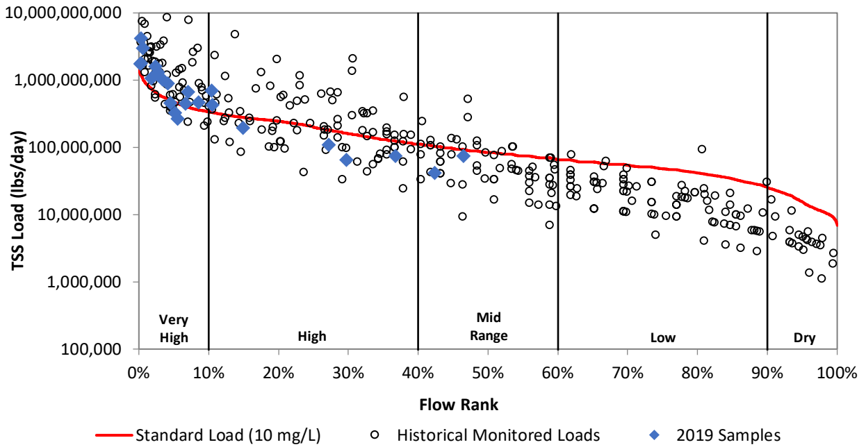
Figure 26f. Load duration curve for total suspended solids at NC801.
