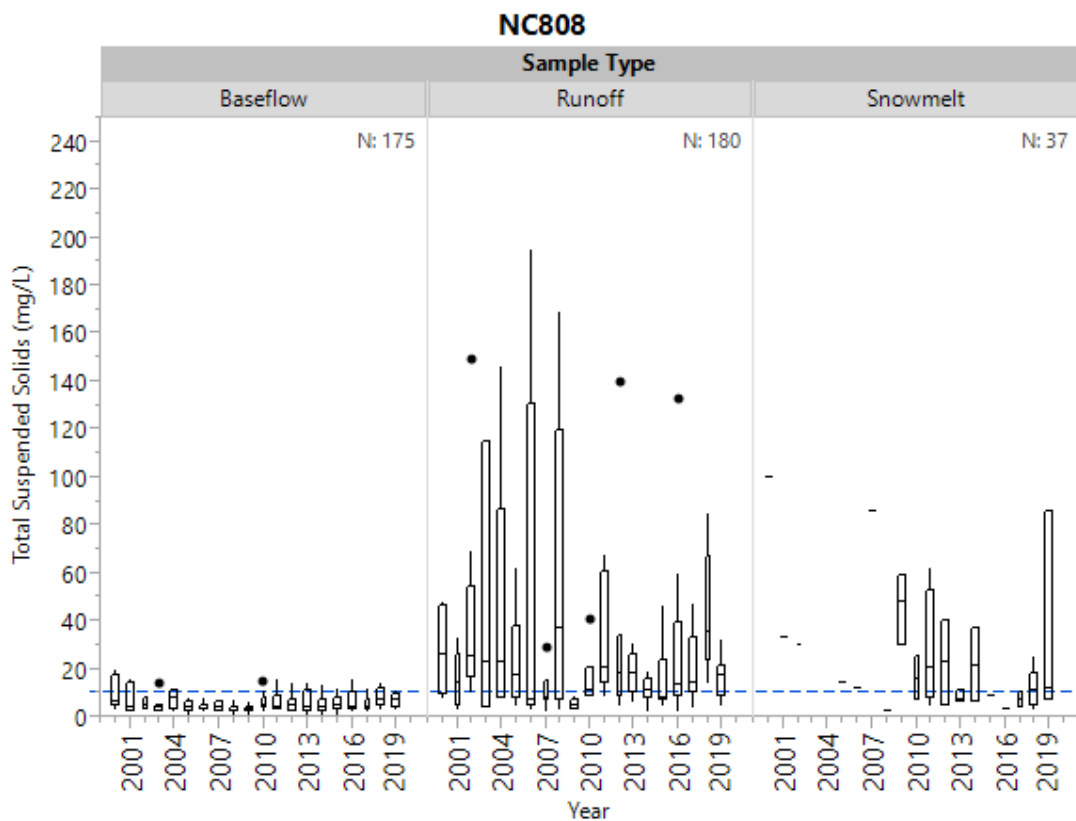
Figure 20e. Historical total suspended solids by sample type at NC808.
