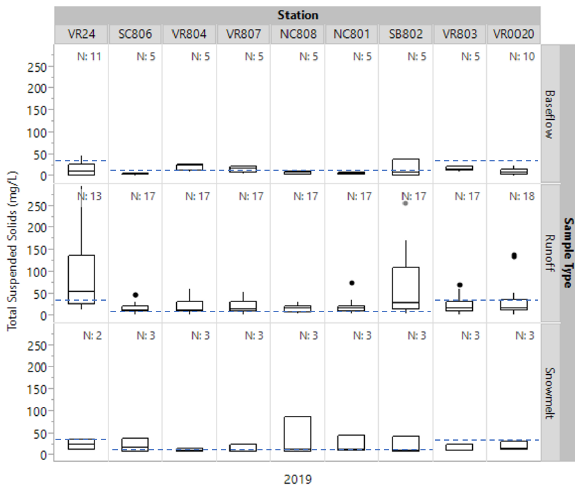
Figure 19. Total suspended solids categorized by sample type for 2019.
