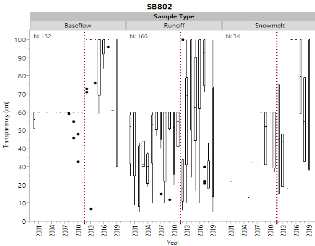
Figure 22g. Historical transparency by sample type for SB802.
