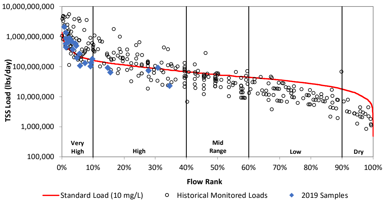
Figure 26e. Load duration curve for total suspended solids at NC808.
