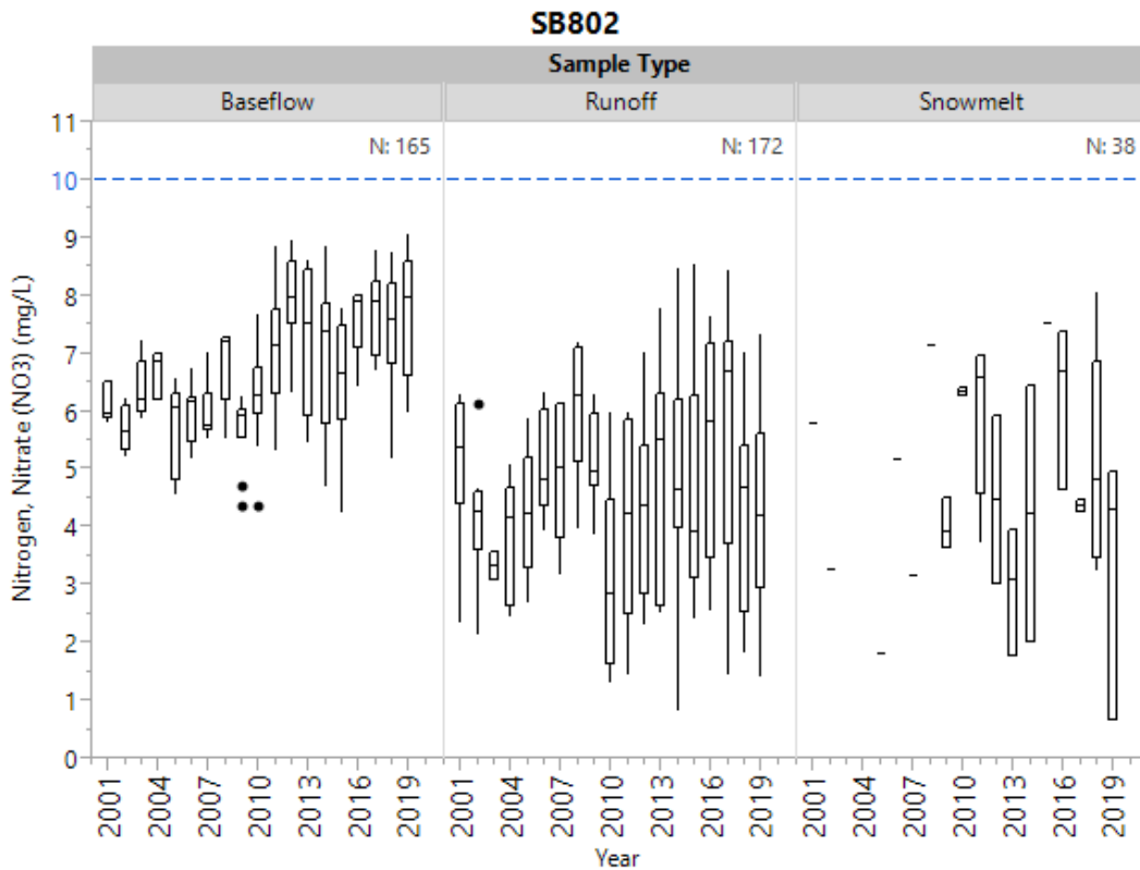
Figure 14g. Historical nitrate by sample type for SB802.
