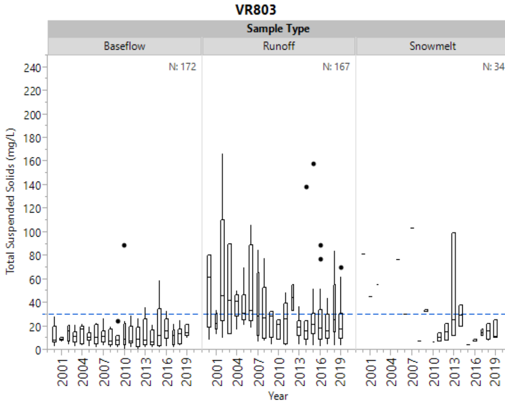
Figure 20h. Historical total suspended solids by sample type at VR803.
