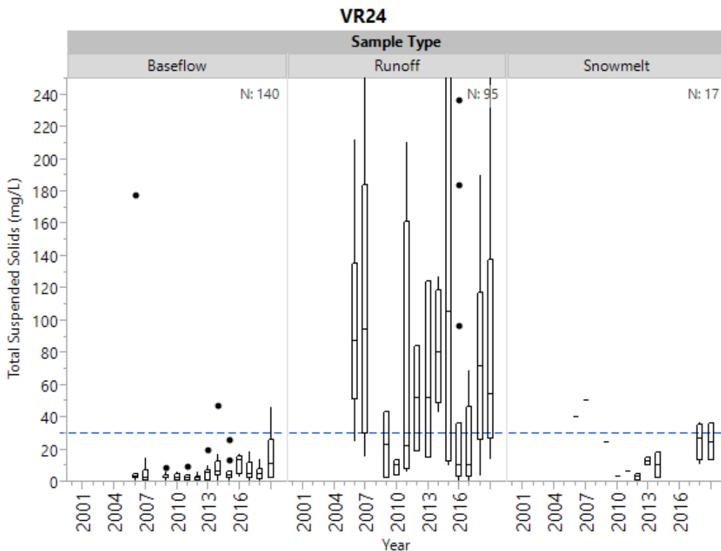
Figure 20a. Historical total suspended solids by sample type at VR24.
