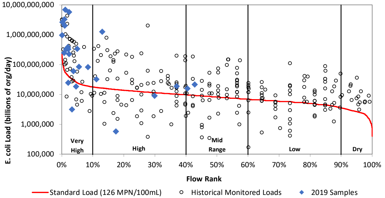
Figure 23g. Load duration curve for E. coli at SB802.
