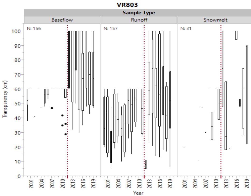
Figure 22h. Historical transparency by sample type for VR803.
