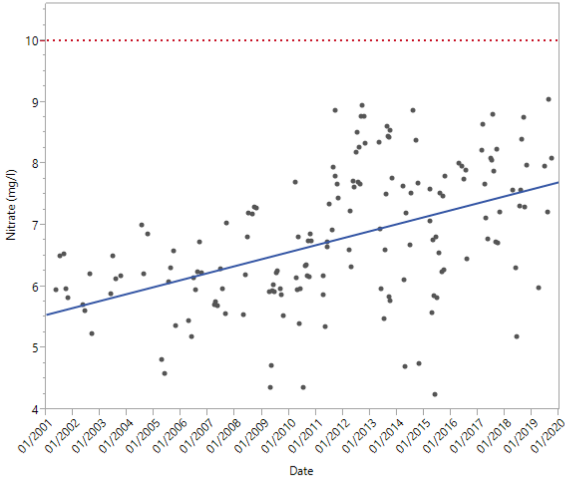
Figure 12. Baseflow nitrate concentration in South Branch Vermillion River, measured at 200th Street East near Highway 52, Dakota County. Samples reflect surface water baseflow conditions (March – October) from 2001 - 2019. Blue solid line represents linear regression. Red dotted line indicates upper limit of state standard, 10 mg/L.
