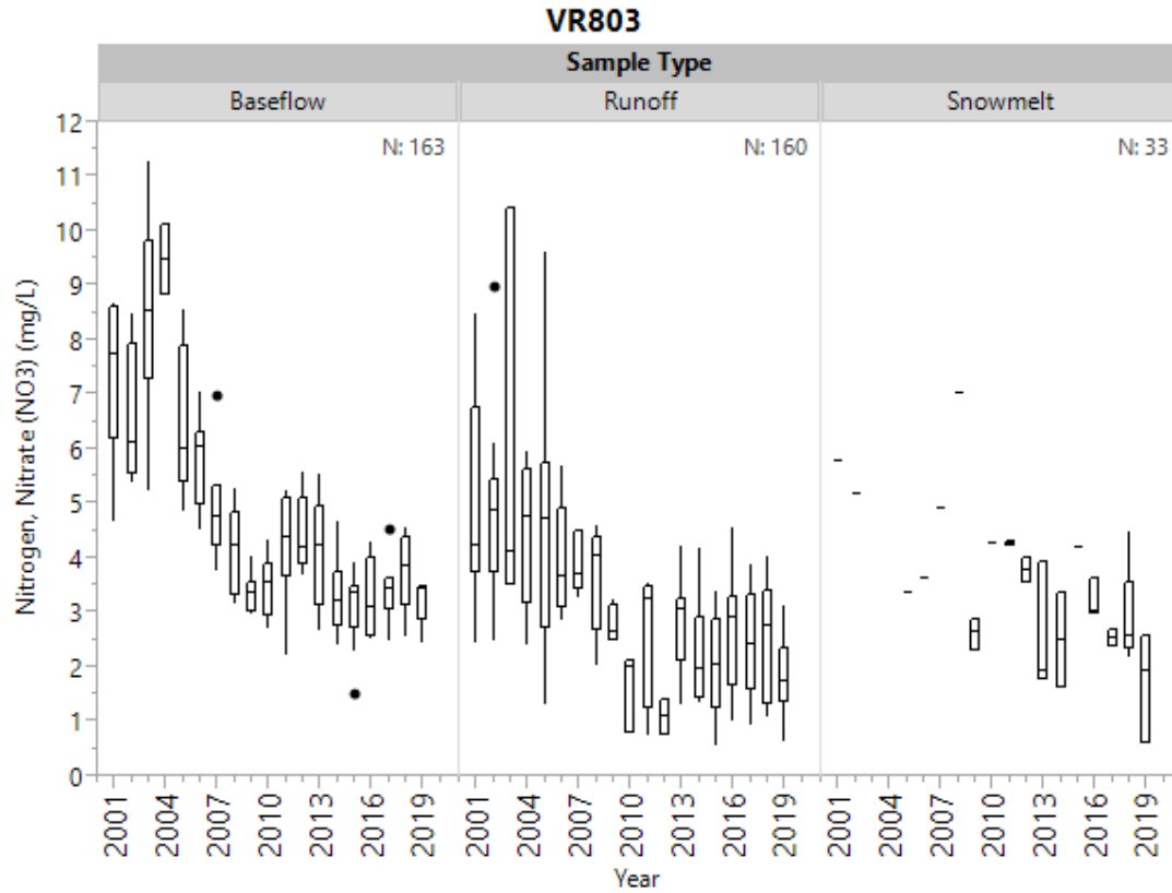
Figure 14h. Historical nitrate by sample type for VR803.
