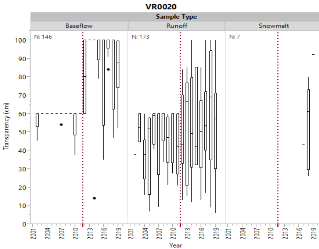
Figure 22i. Historical transparency by sample type for VR0020.
