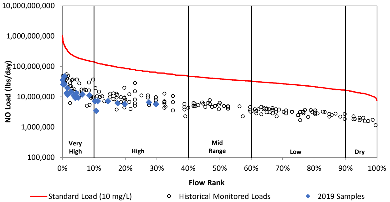
Figure 24b. Load duration curve for nitrate at SC806.
