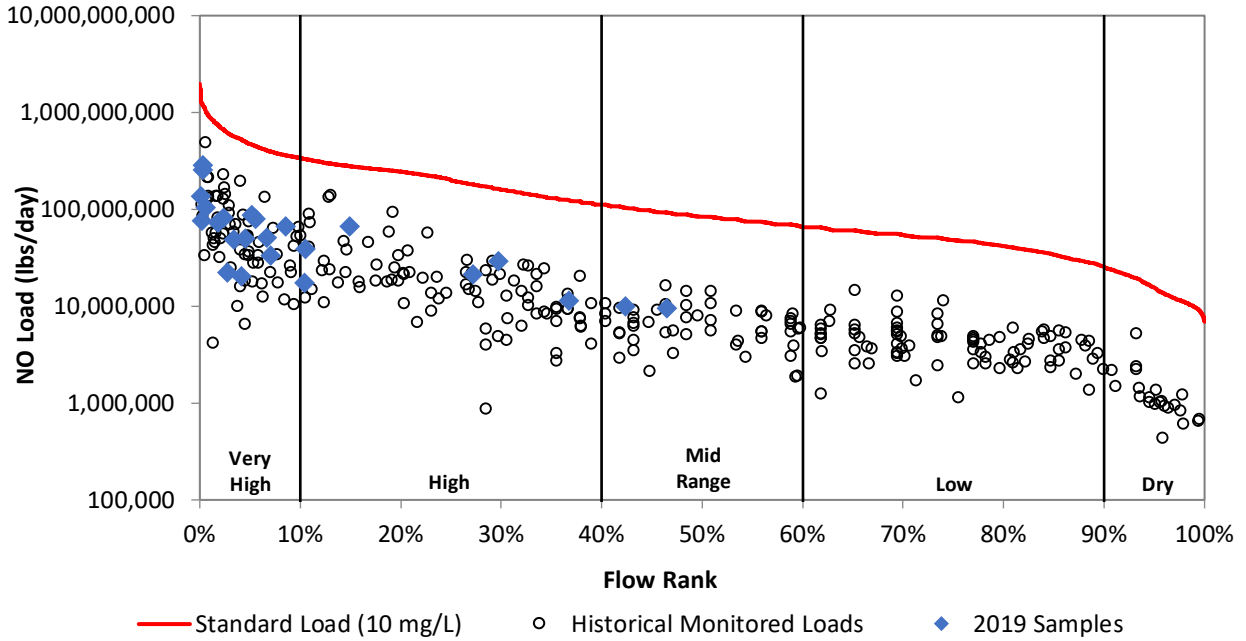
Figure 24f. Load duration curve for nitrate at NC801.
