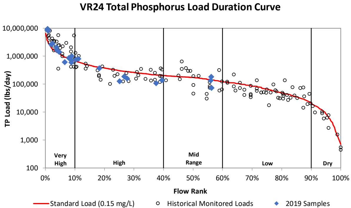
Figure 25a. Load duration curve for total phosphorus at VR24.
