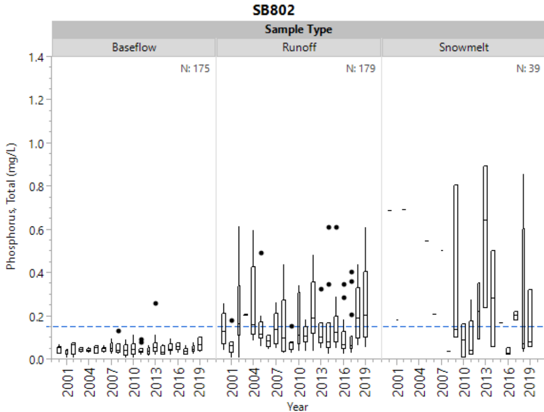
Figure 16g. Historical total phosphorus by sample type at SB802.
