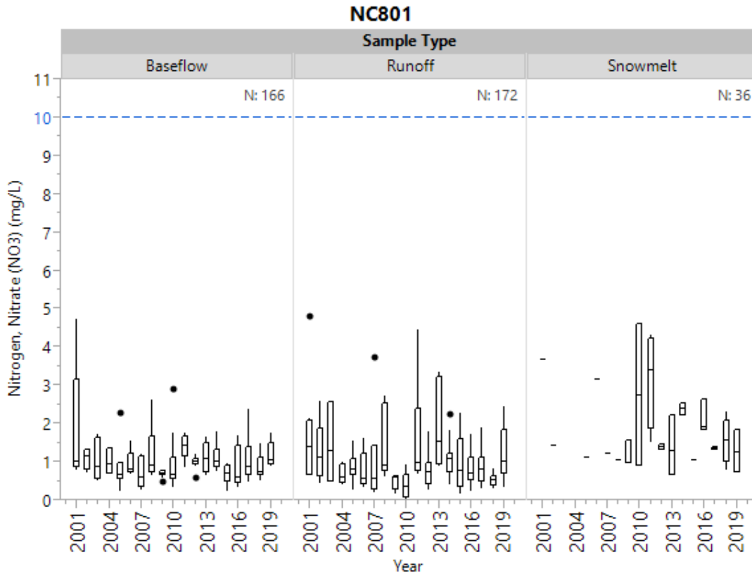
Figure 14f. Historical nitrate by sample type for NC801.
