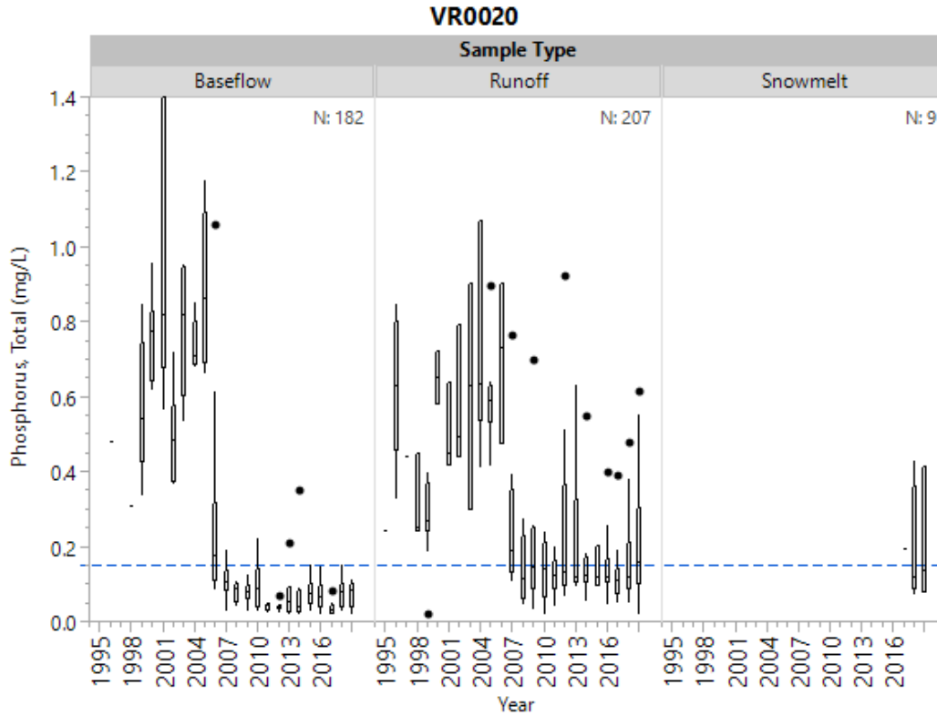
Figure 16i. Historical total phosphorus by sample type at VR0020. **VR0020 maximum for 2001 baseflow sample extends to 4 mg/L.
