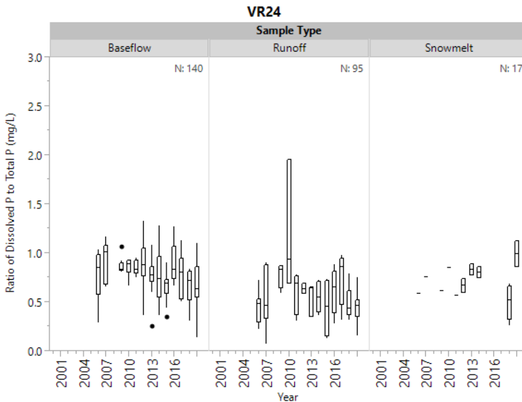
Figure 18a. Historical ratio of dissolved phosphorus to total phosphorus by sample type at VR24.
