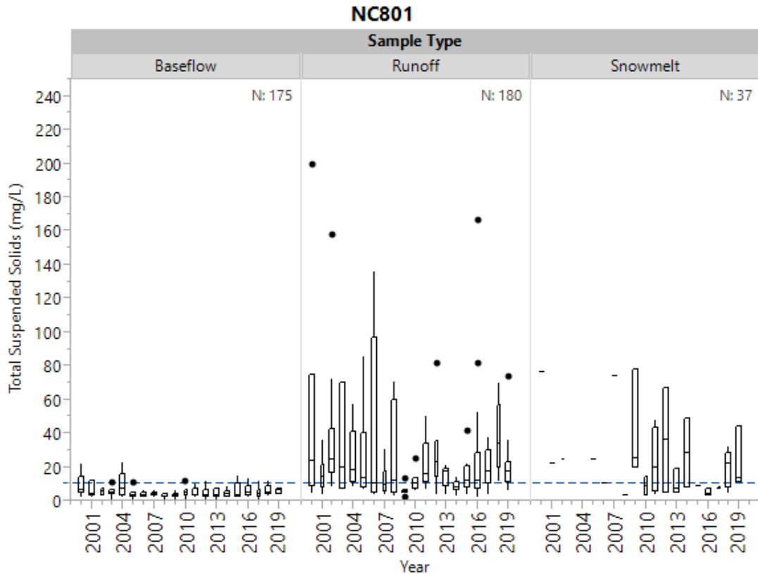
Figure 20f. Historical total suspended solids by sample type at NC801.
