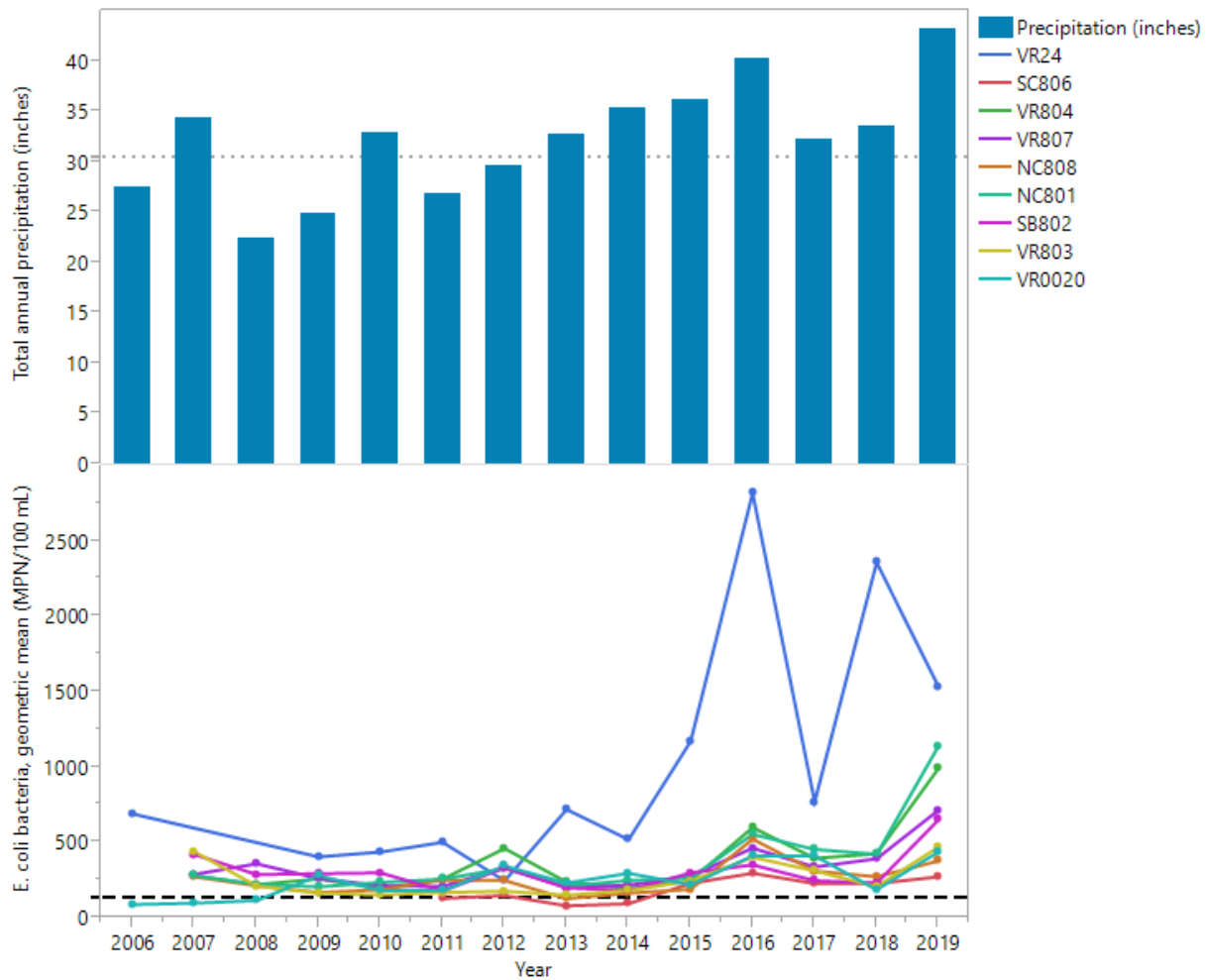
Figure 11. Annual geometric mean of Escherichia coli (E. coli) bacteria for all stations by year. MPN stands for most probable number of organisms. Black dashed line indicates the 30-day geometric mean standard (for data collected April through October) of \leq 126 MPN/100 mL. Bars represent total annual precipitation for each year. Gray dotted line indicates the 30 year (1989-2018) total annual average precipitation at the Minneapolis – St. Paul airport weather station of 31 inches.
