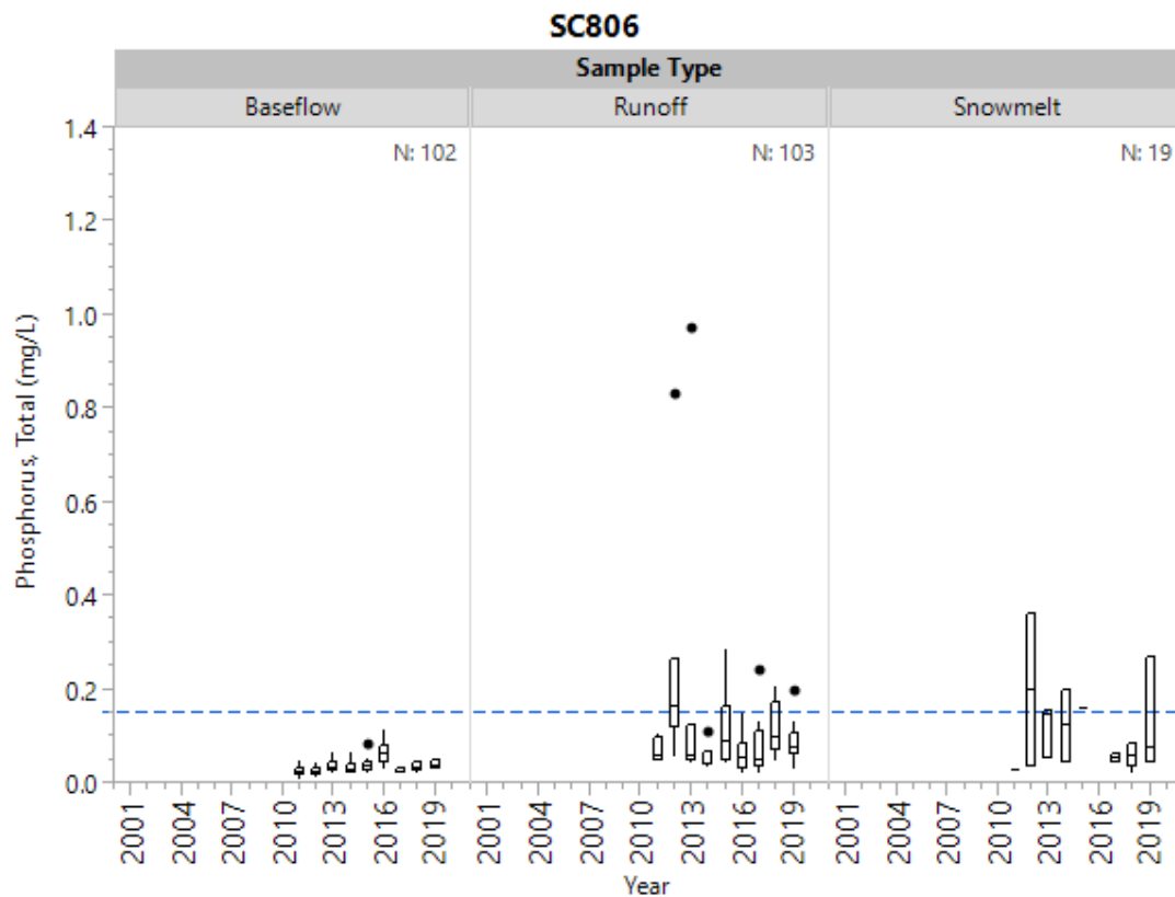
Figure 16b. Historical total phosphorus by sample type at SC806.
