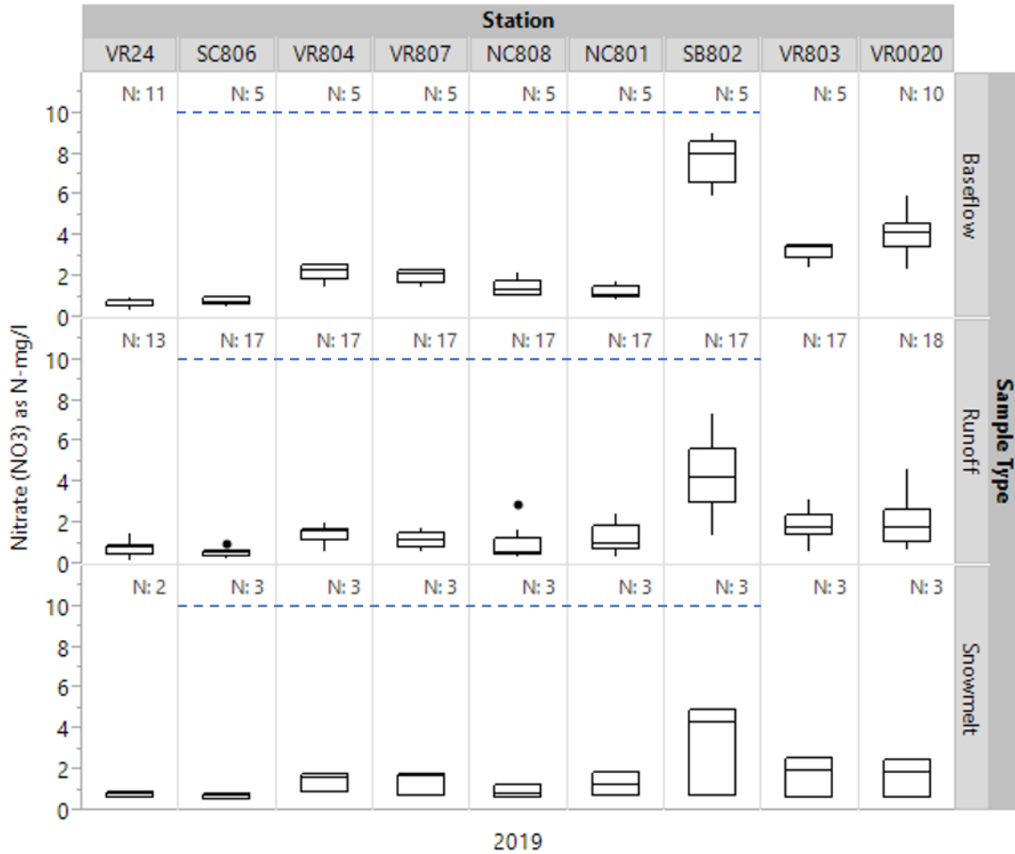
Figure 13. Nitrate nitrogen for each station, categorized by sample type, for 2019. .
