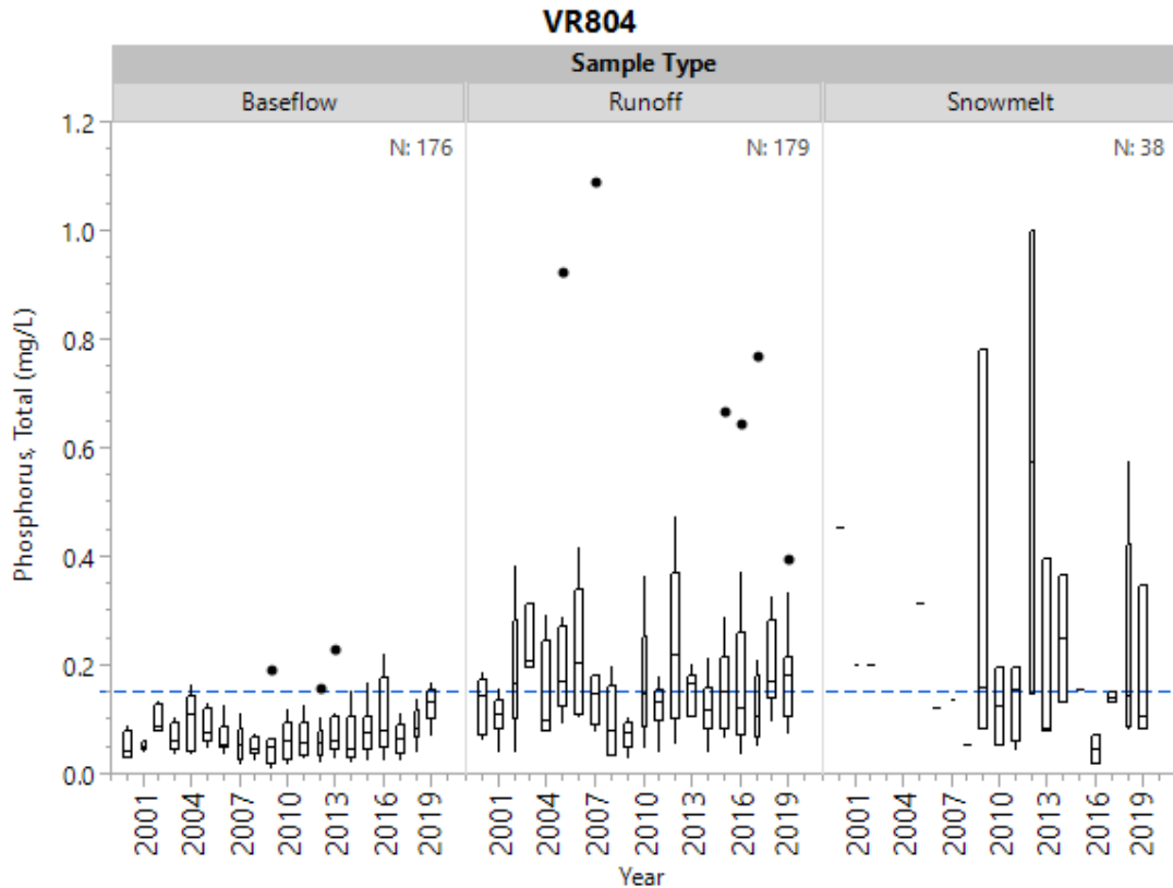
Figure 16c. Historical total phosphorus by sample type at VR804.
