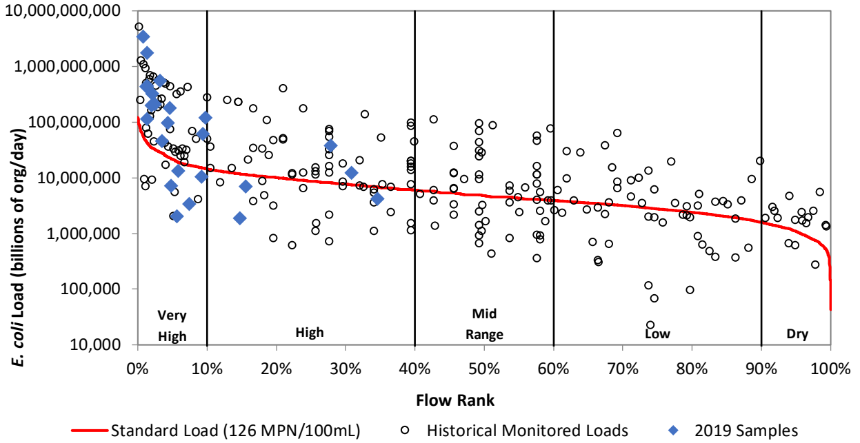
Figure 23e. Load duration curve for E. coli at NC808.
