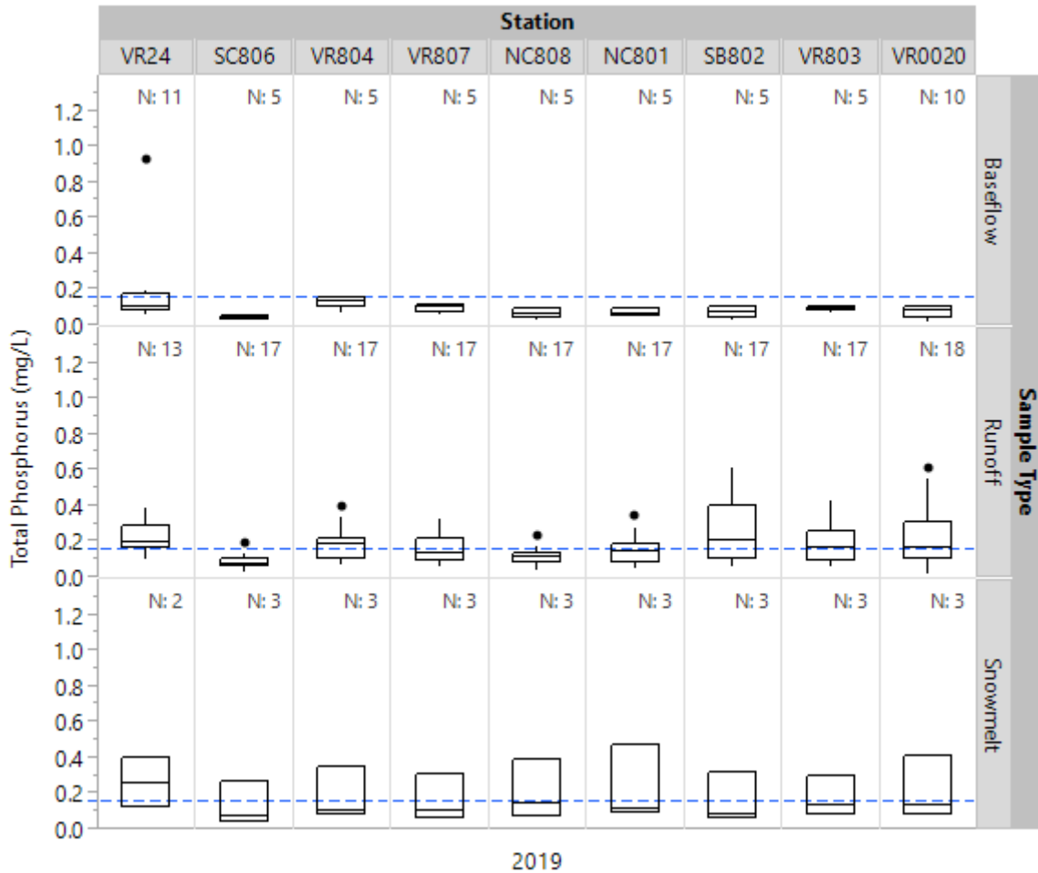
Figure 15. Total phosphorus (TP) for each station, categorized by sample type, for 2019.
