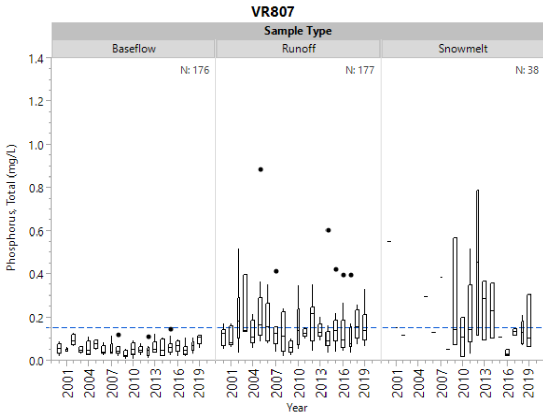
Figure 16d. Historical total phosphorus by sample type at VR807.
