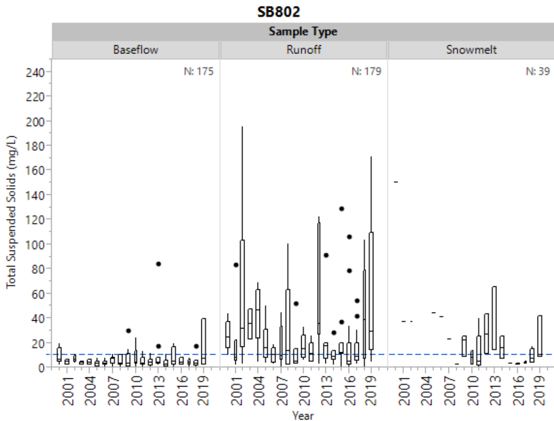
Figure 20g. Historical total suspended solids by sample type at SB802.
