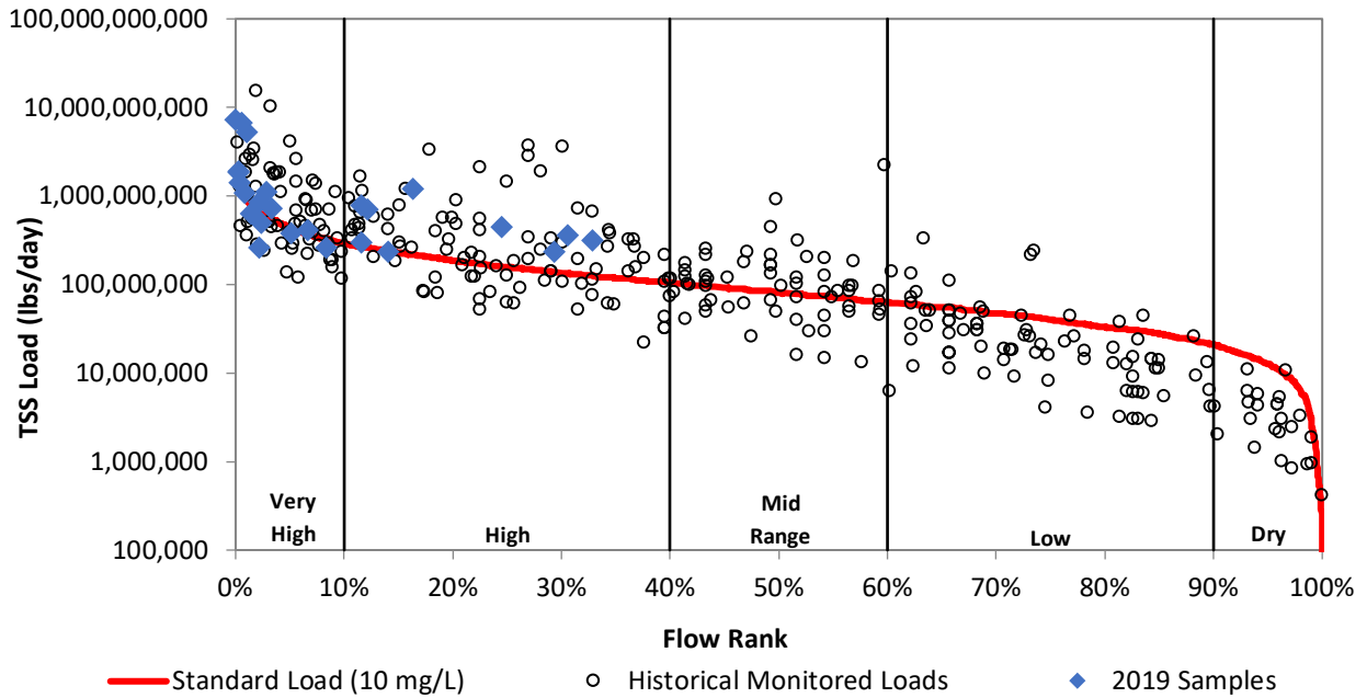
Figure 26c. Load duration curve for total suspended solids at VR804.
