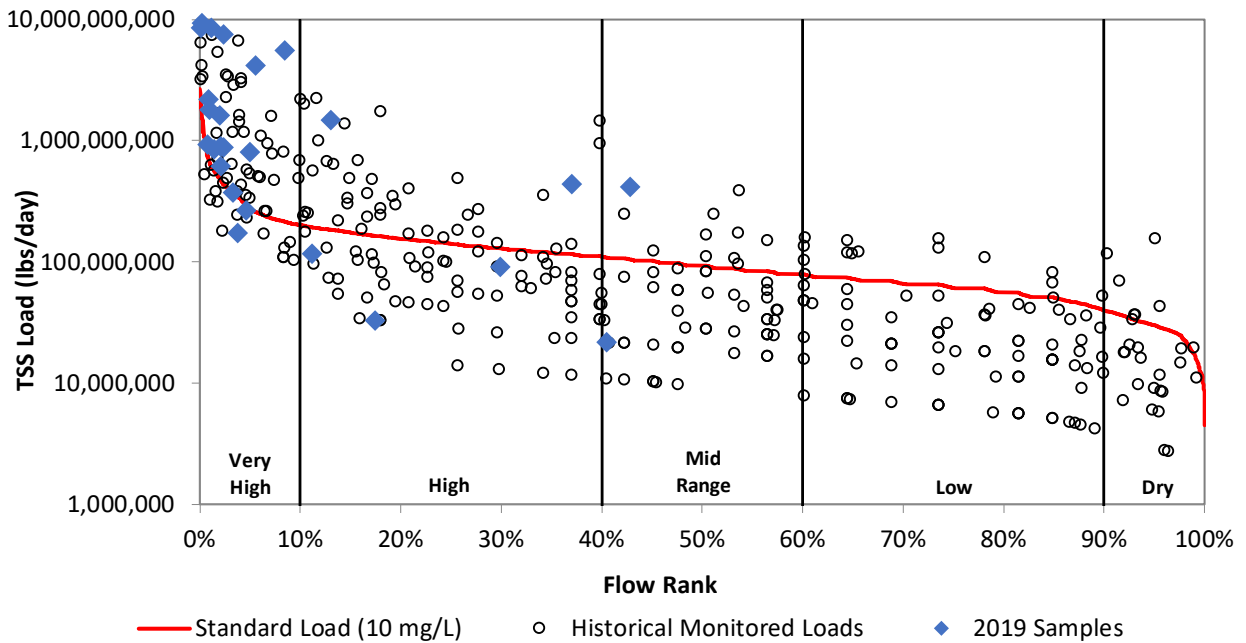
Figure 26g. Load duration curve for total suspended solids at SB802.
