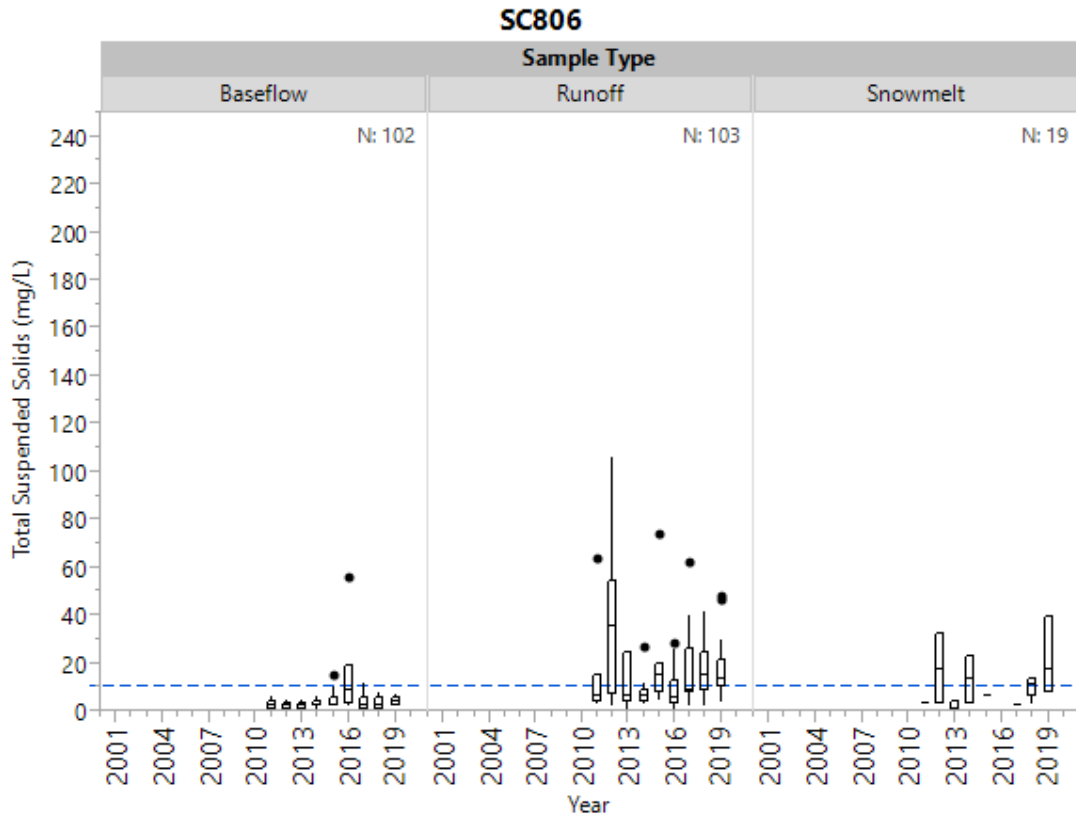
Figure 20b. Historical total suspended solids by sample type at SC806.
