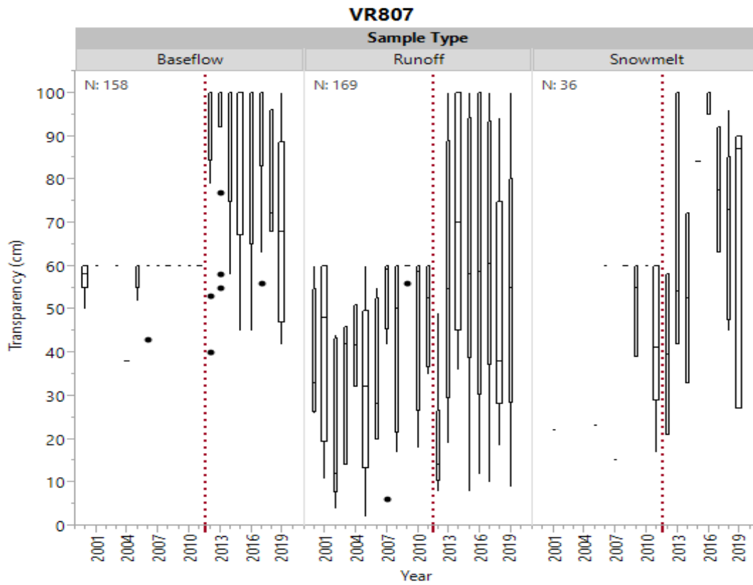
Figure 22d. Historical transparency by sample type for VR807.
