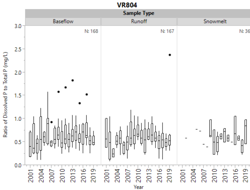
Figure 18c. Historical ratio of dissolved phosphorus to total phosphorus by sample type at VR804.
