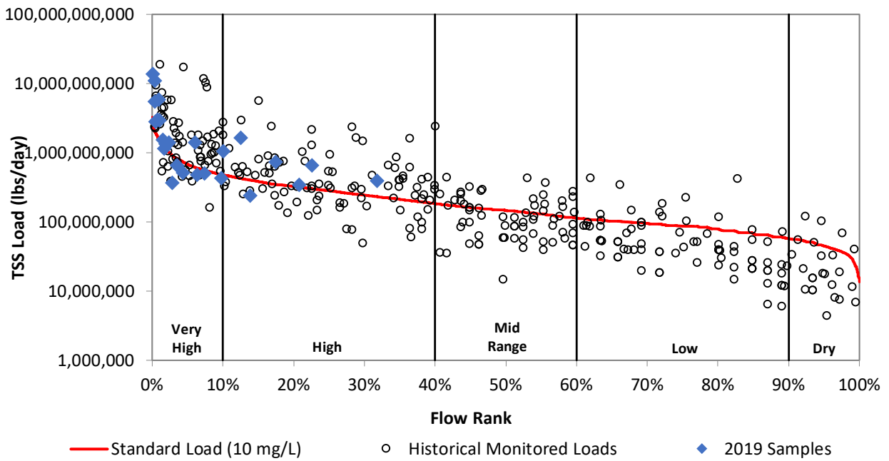
Figure 26d. Load duration curve for total suspended solids at VR807.
