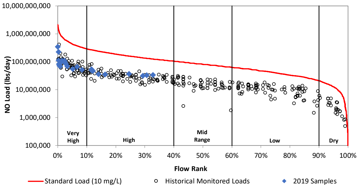
Figure 24c. Load duration curve for nitrate at VR804.
