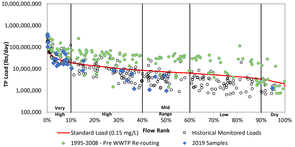
Figure 25i. Load duration curve for total phosphorus at VR0020.
