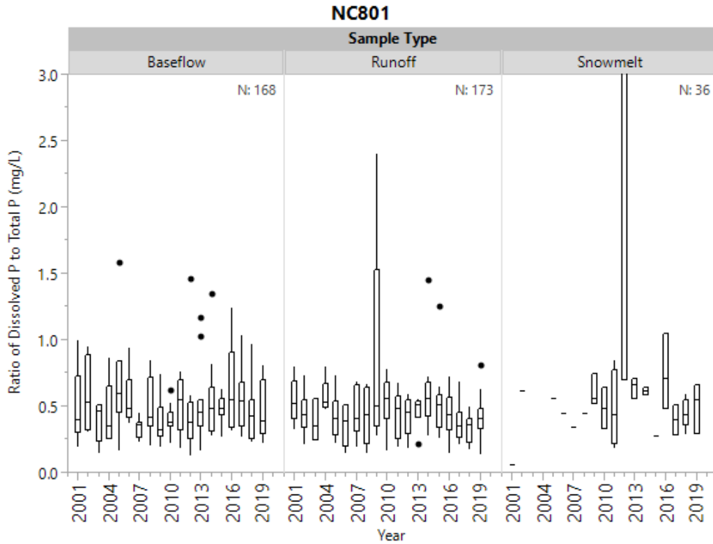
Figure 18f. Historical ratio of dissolved phosphorus to total phosphorus by sample type at NC801. **NC801 has an outlier for 2003 baseflow at 3.7 mg/L and the maximum for 2012 snowmelt sample extends to 5.67 mg/L.
