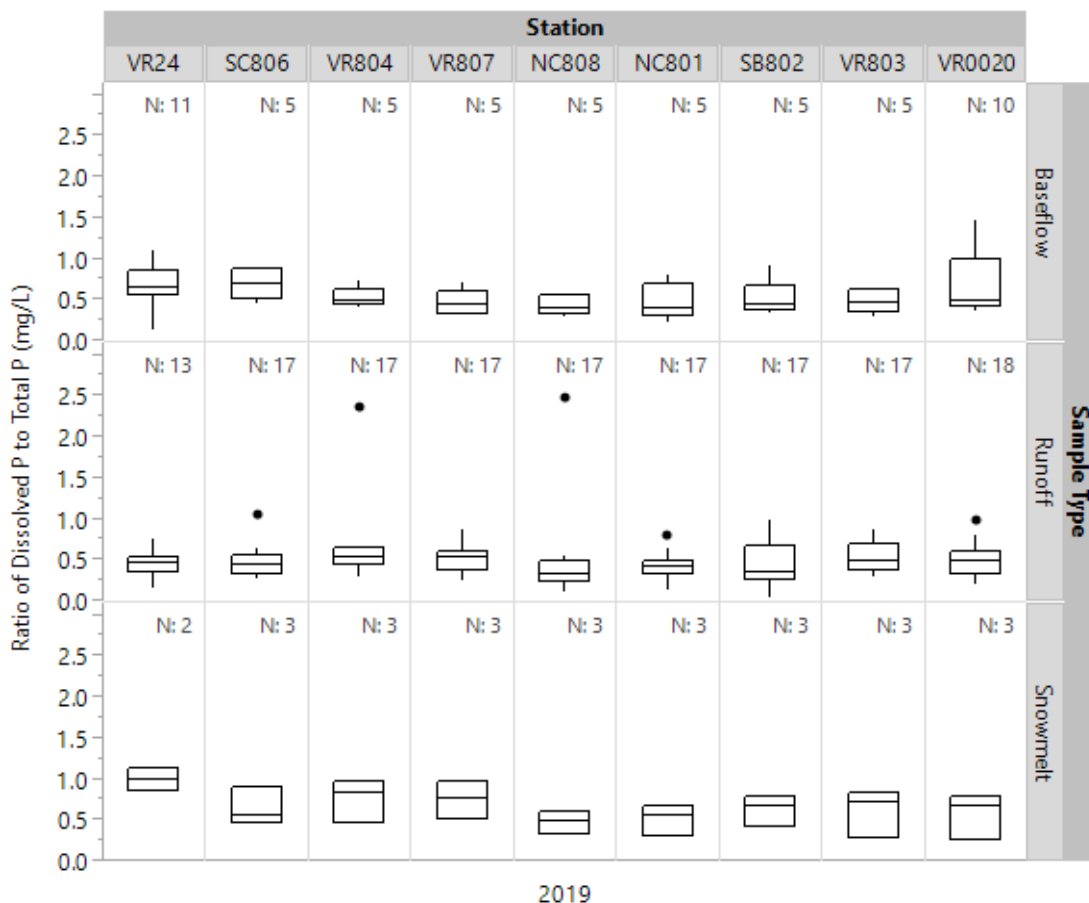
Figure 17. Ratio of dissolved phosphorus (TDP) to total phosphorus (TP) for each station, categorized by sample type, for 2019.
