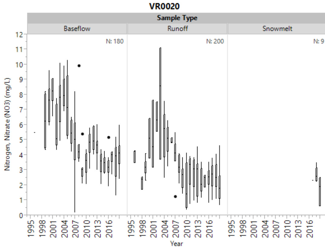
Figure 14i. Historical nitrate by sample type for VR0020.
