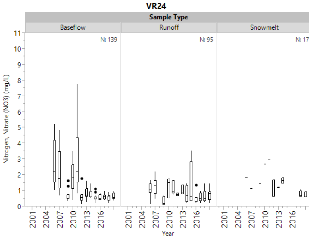
Figure 14a. Historical nitrate by sample type for VR24.
