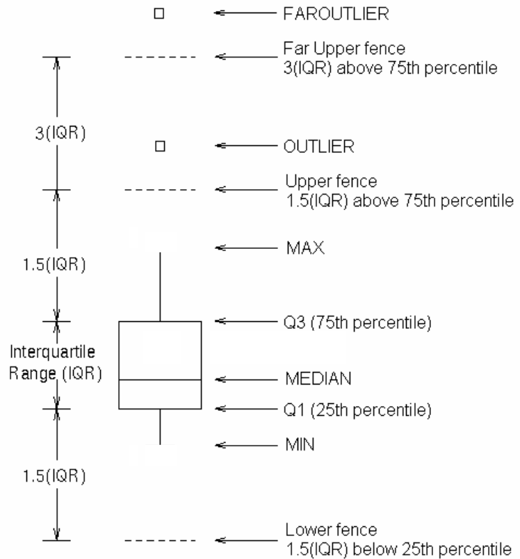
Figure 2. Vertical boxplot display key.
