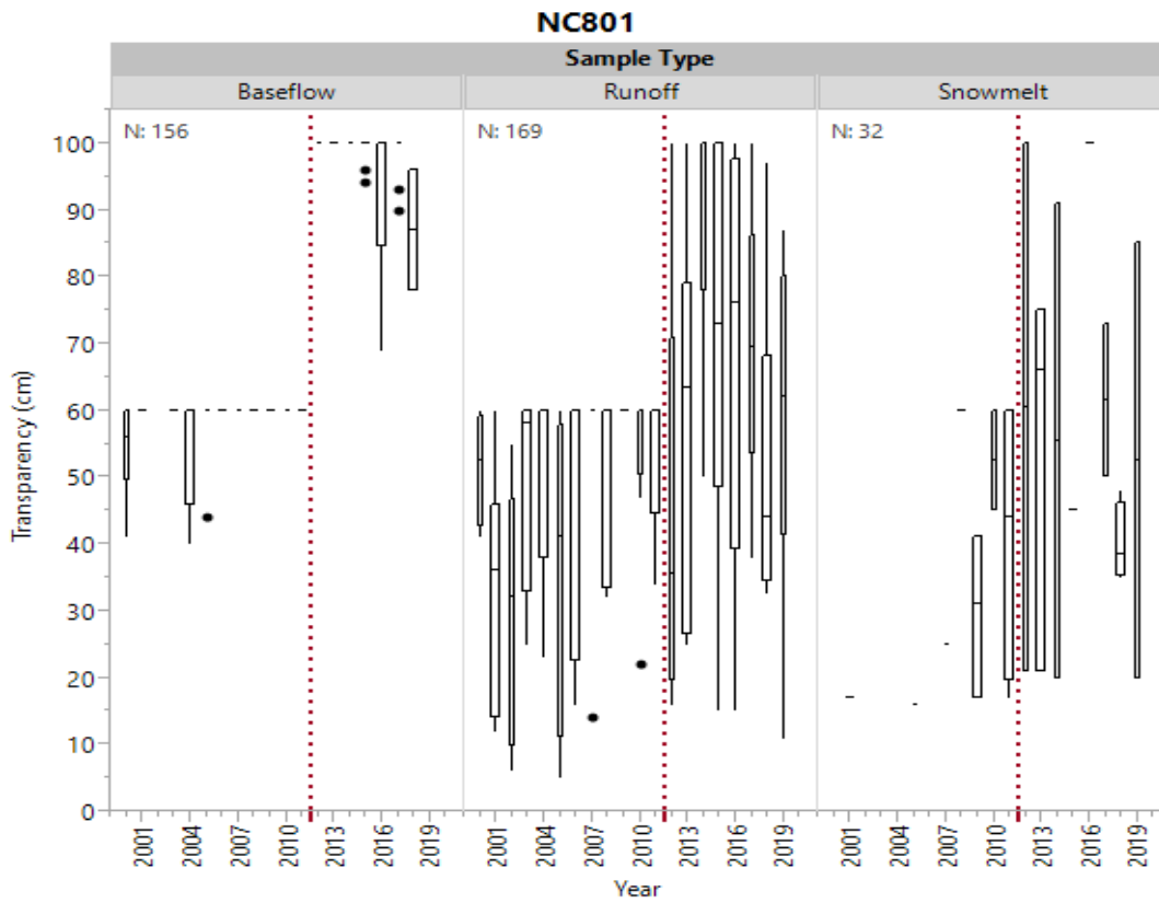
Figure 22f. Historical transparency by sample type for NC801.
