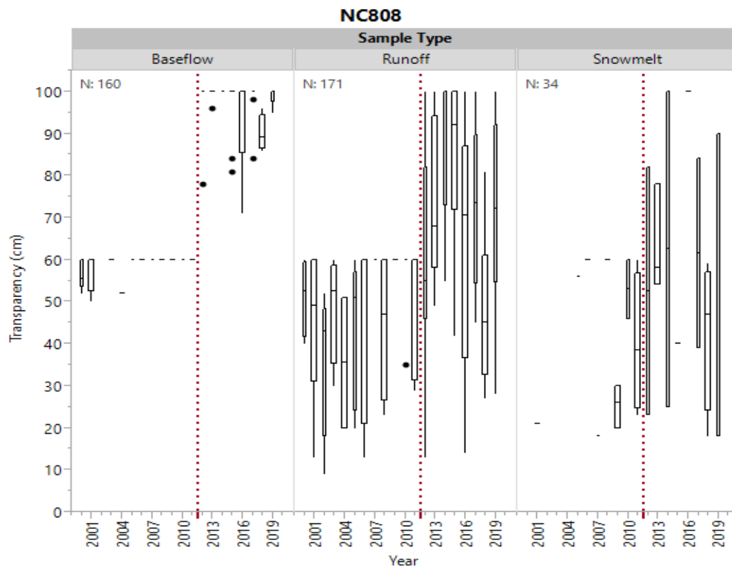
Figure 22e. Historical transparency by sample type for NC808.
