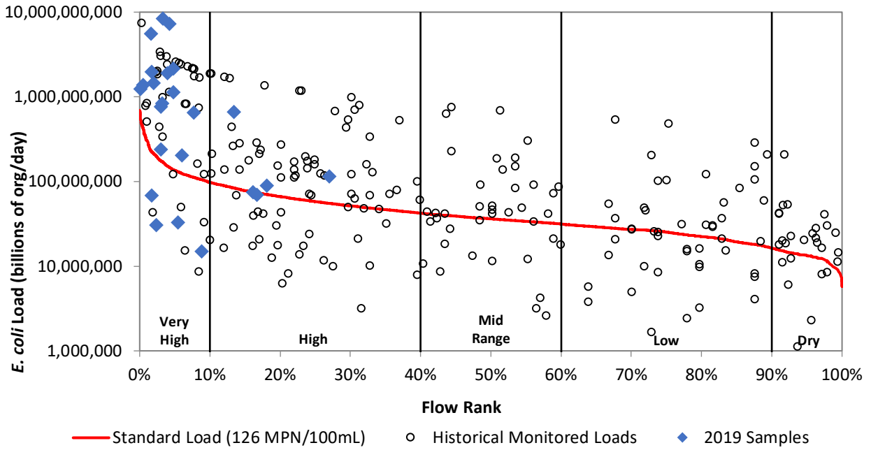
Figure 23h. Load duration curve for E. coli at VR803.
