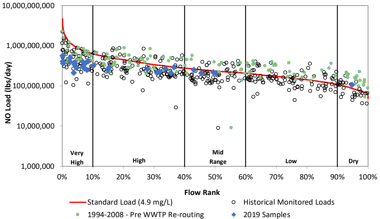
Figure 24i. Load duration curve for nitrate at VR0020.
