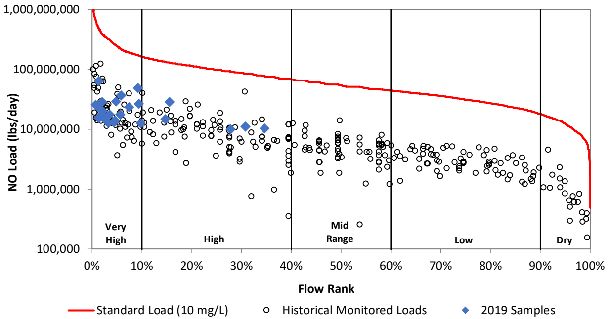
Figure 24e. Load duration curve for nitrate at NC808.
