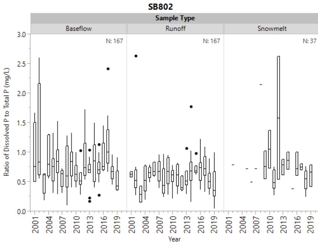
Figure 18g. Historical ratio of dissolved phosphorus to total phosphorus by sample type at SB802.
