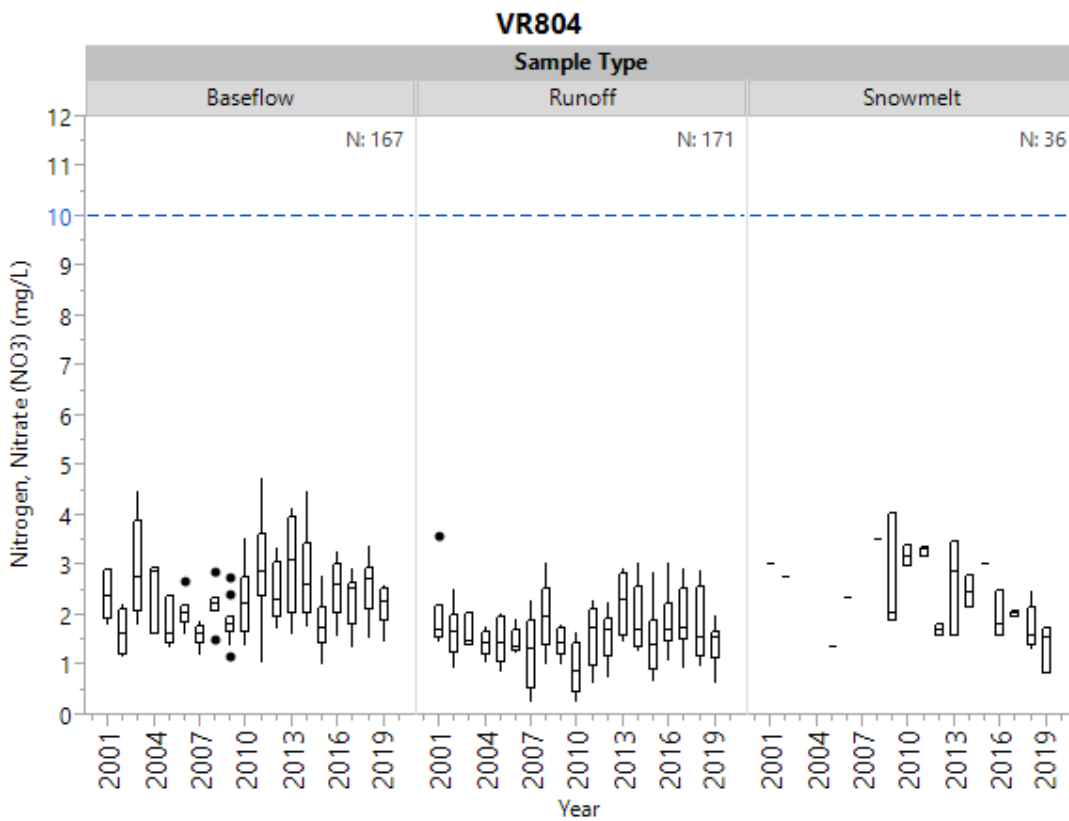
Figure 14c. Historical nitrate by sample type for VR804.
