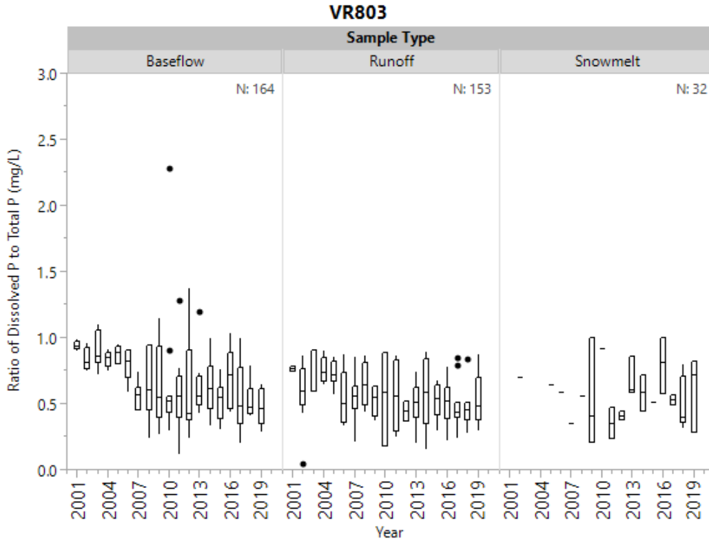
Figure 18h. Historical ratio of dissolved phosphorus to total phosphorus by sample type at VR803.
