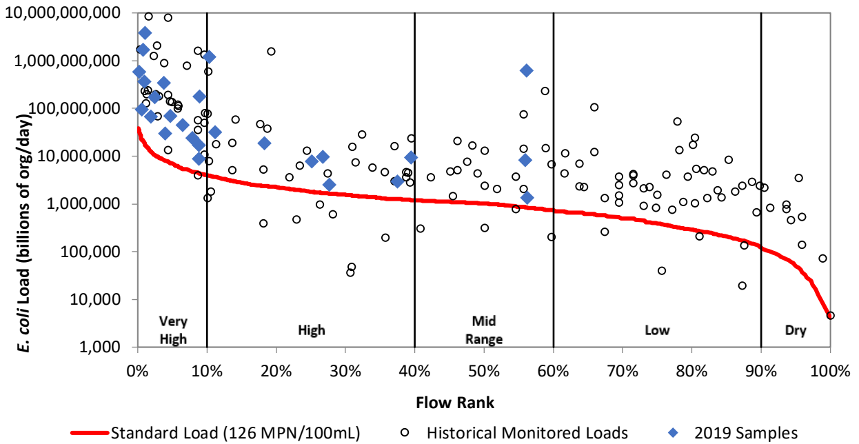
Figure 23a. Load duration curve for E. coli at VR24.
