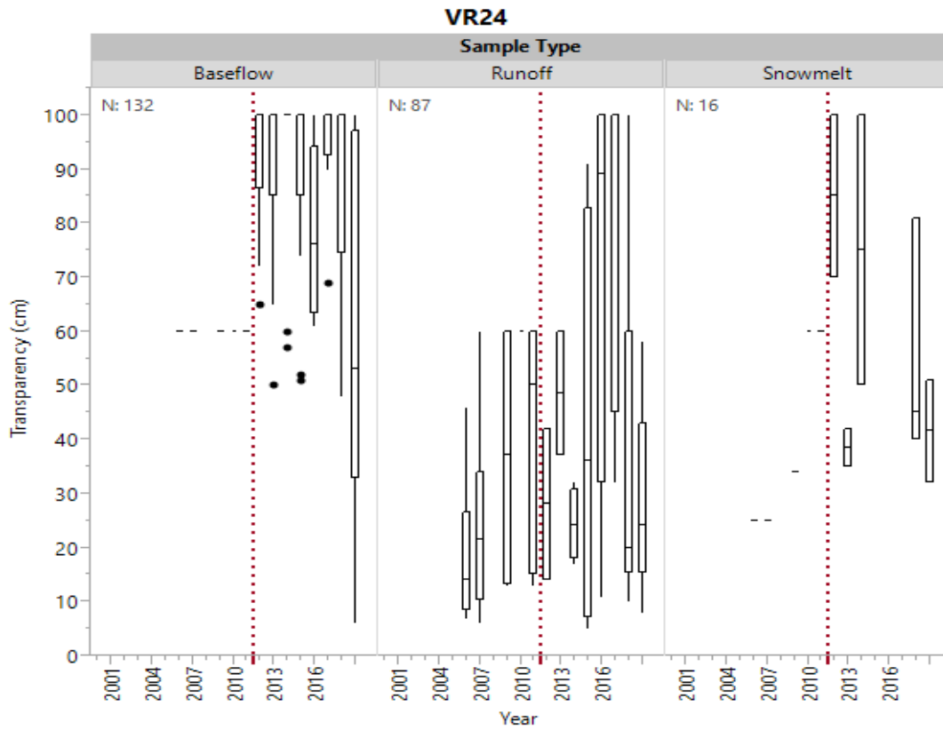
Figure 22a. Historical transparency by sample type for VR24.
