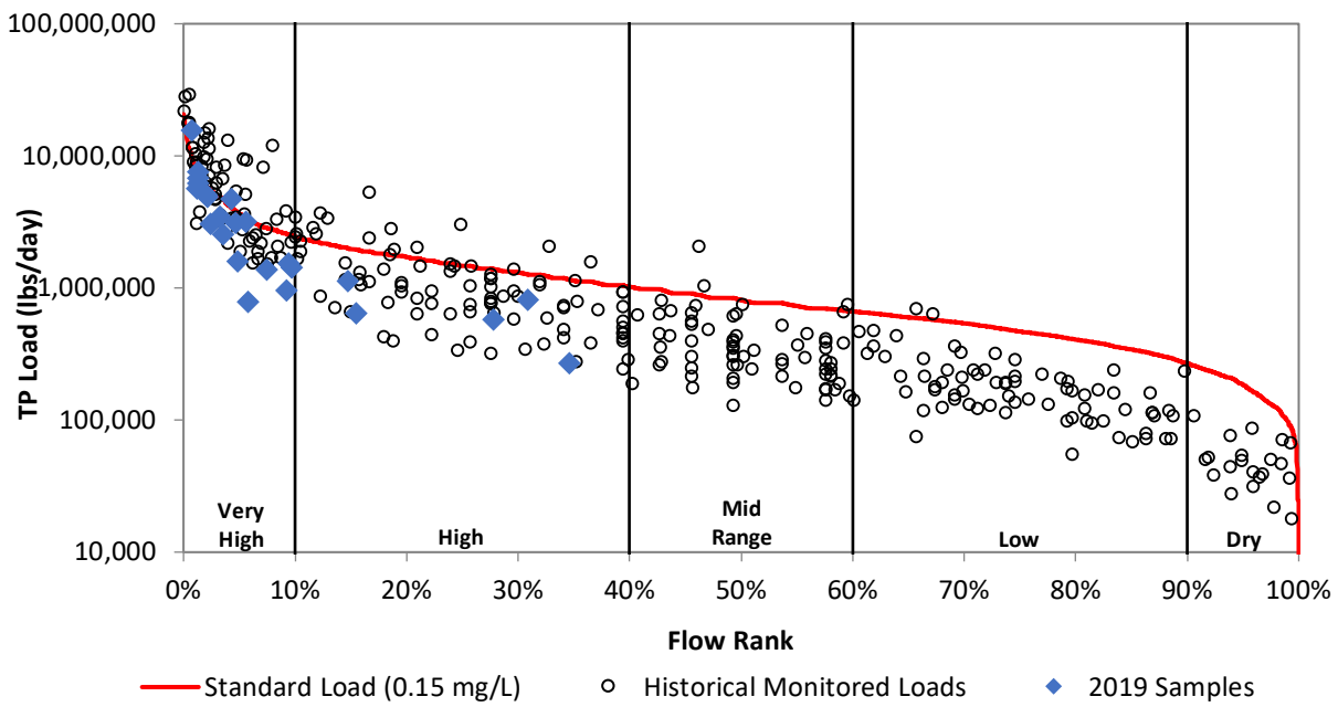
Figure 25e. Load duration curve for total phosphorus at NC808.
