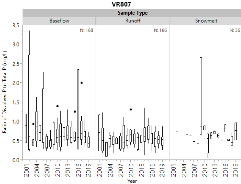
Figure 18d. Historical ratio of dissolved phosphorus to total phosphorus by sample type at VR807.
