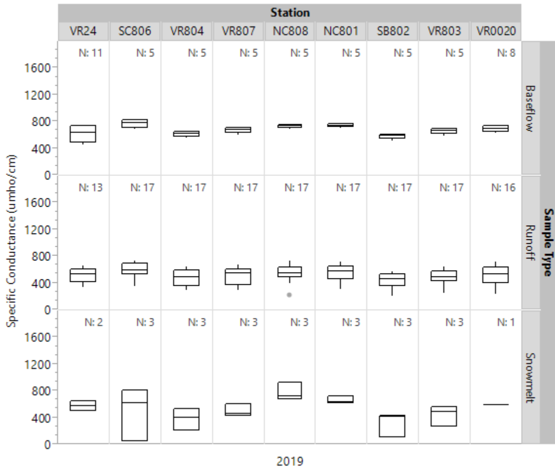
Figure 6. Specific conductance for each station, categorized by sample type, for 2019.
