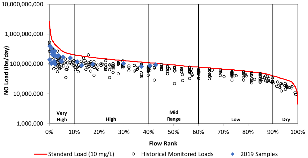
Figure 24g. Load duration curve for nitrate at SB802.
