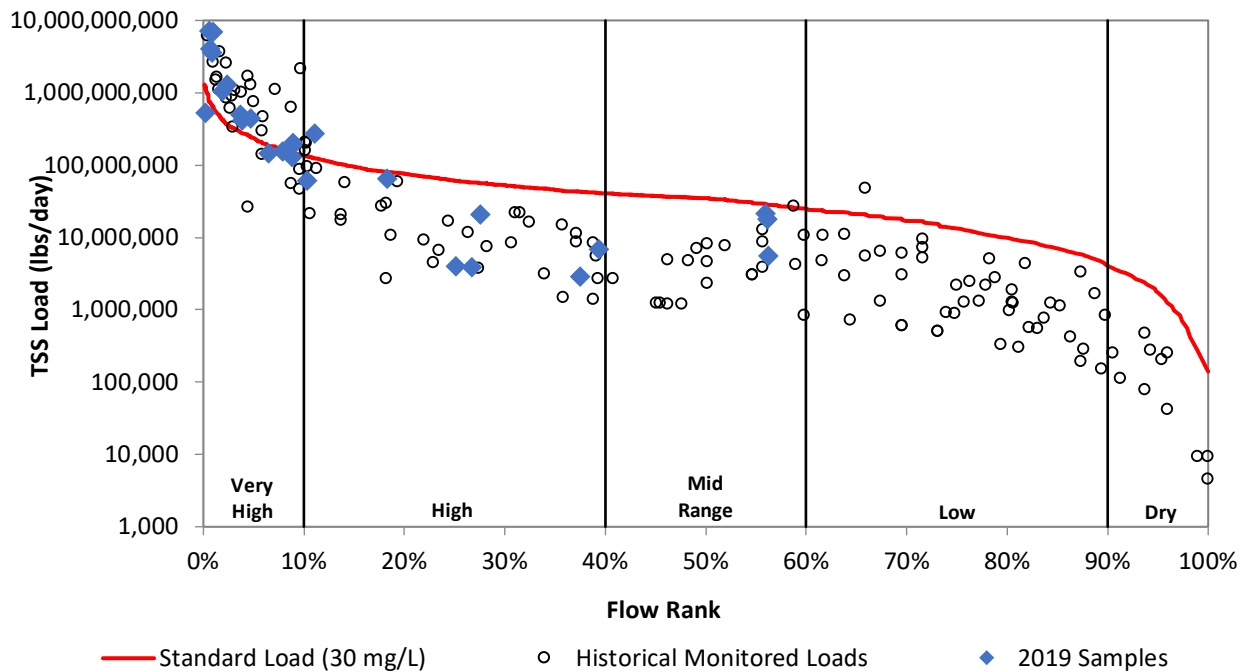
Figure 26a. Load duration curve for total suspended solids at VR24.
