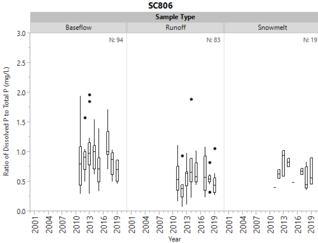
Figure 18b. Historical ratio of dissolved phosphorus to total phosphorus by sample type at SC806.
