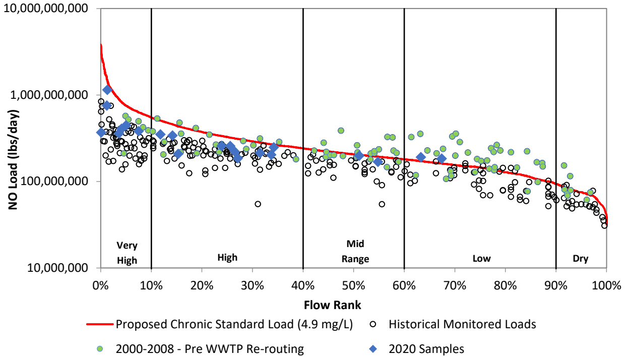
Figure 26h. Load duration curve for nitrate at VR803.
