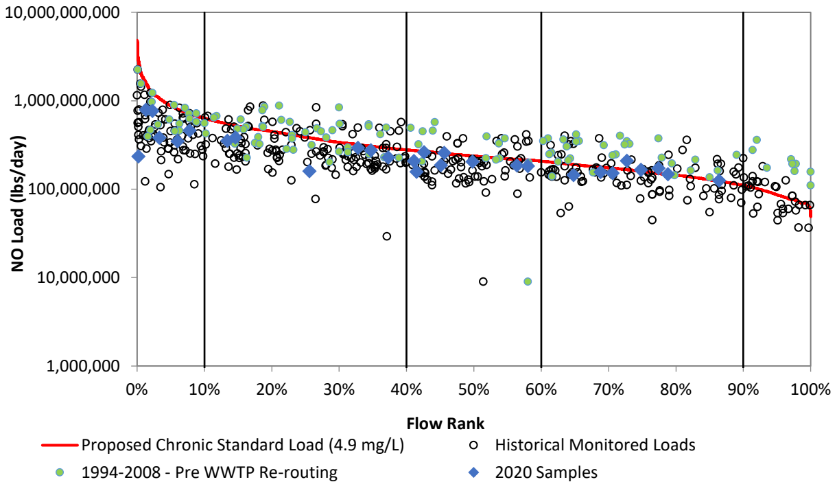
Figure 26i. Load duration curve for nitrate at VR0020.
