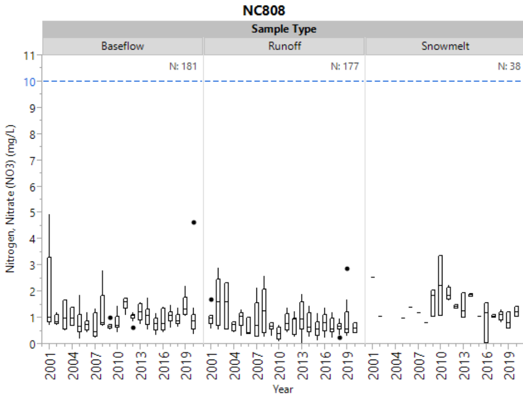
Figure 16e. Historical nitrate by sample type for NC808.
