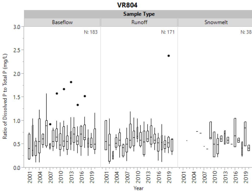
Figure 20c. Historical ratio of dissolved phosphorus to total phosphorus by sample type at VR804.
