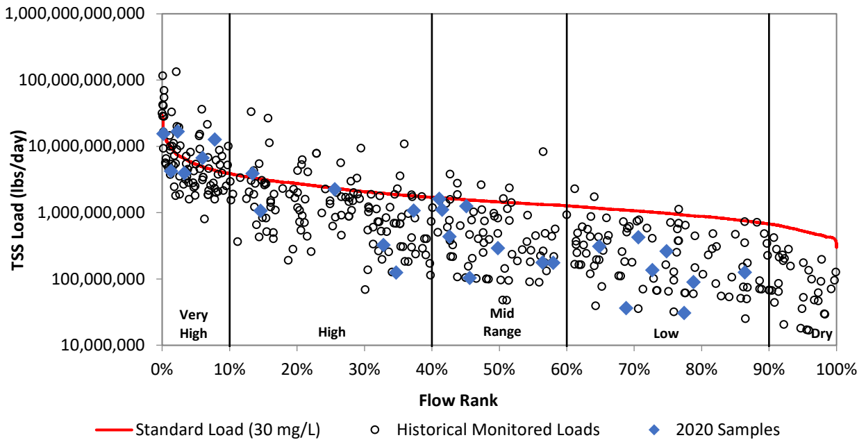
Figure 28i. Load duration curve for total suspended solids at VR0020.
