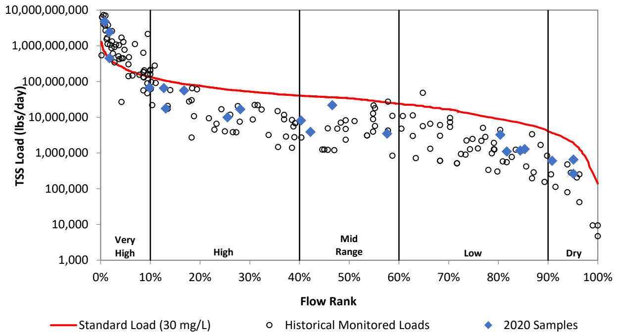
Figure 28a. Load duration curve for total suspended solids at VR24.
