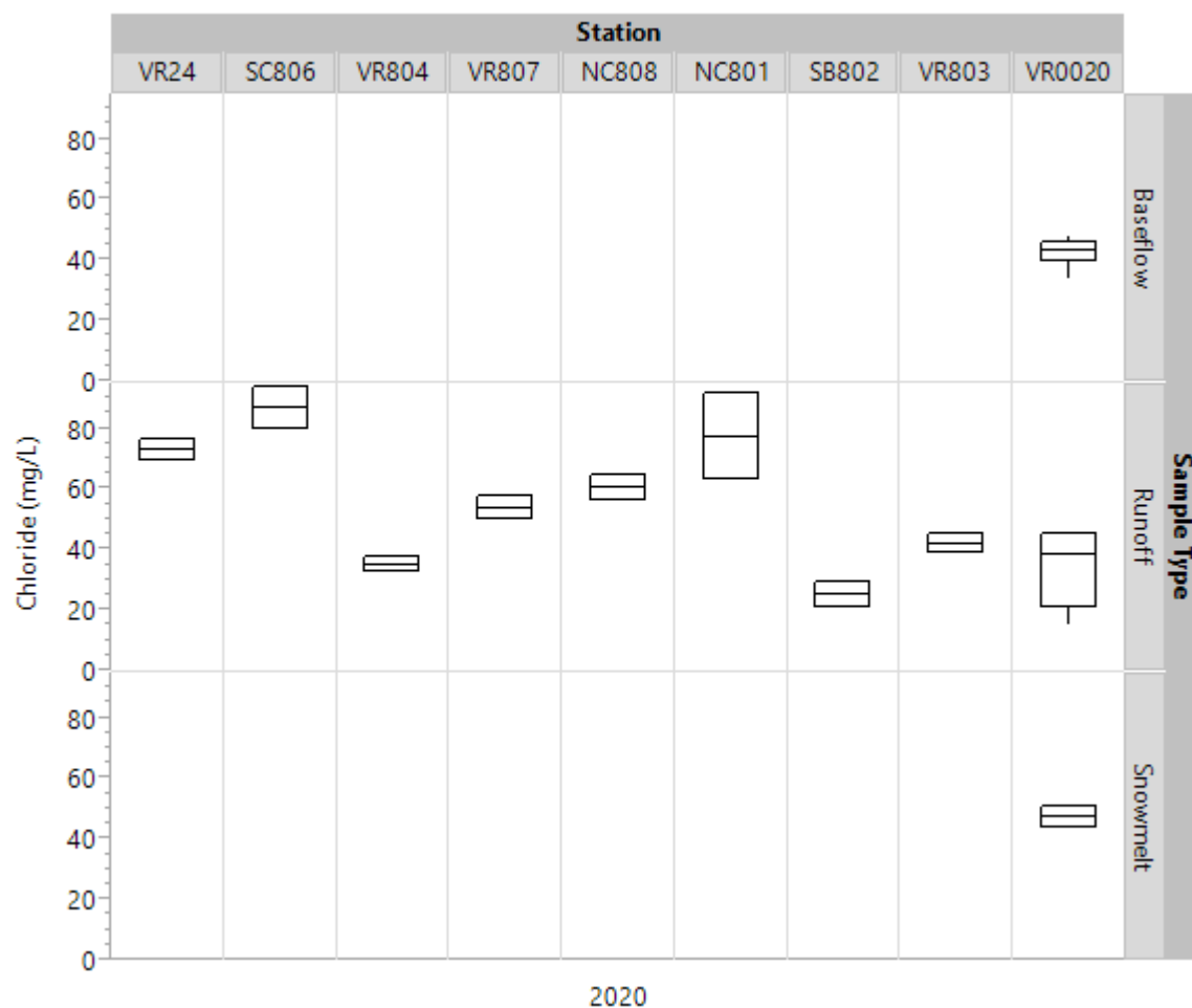
Figure 11. Chloride for each station for 2020.
