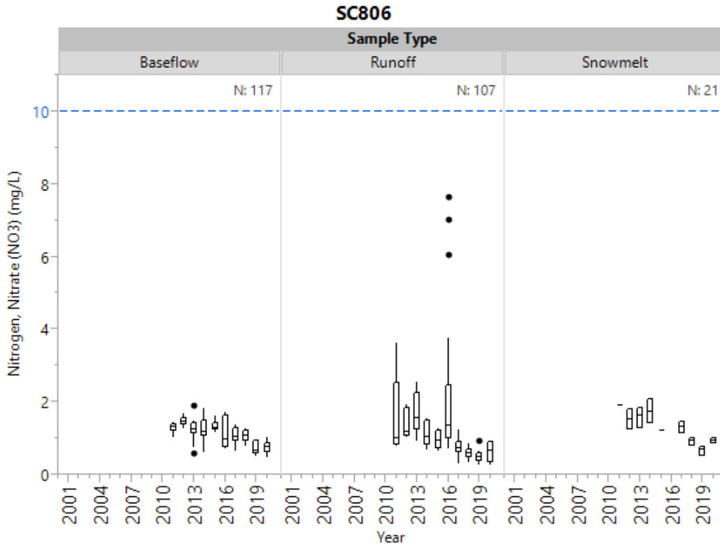
Figure 16b. Historical nitrate by sample type for SC806.
