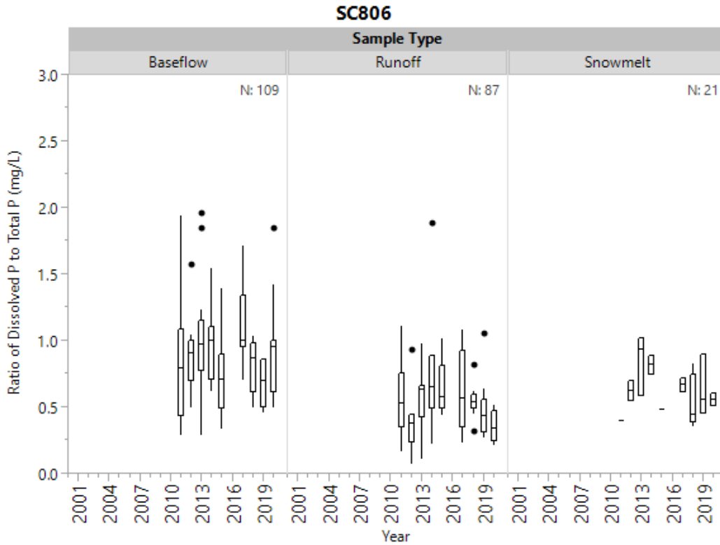
Figure 20b. Historical ratio of dissolved phosphorus to total phosphorus by sample type at SC806.
