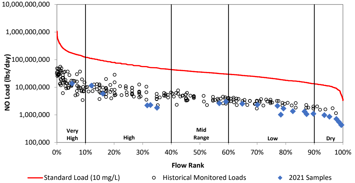
Figure 26b. Load duration curve for nitrate at SC806.
