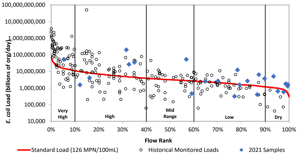
Figure 25b. Load duration curve for E. coli at SC806.
