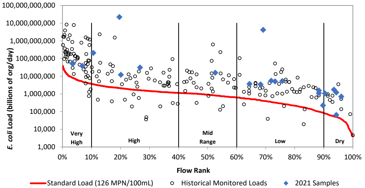
Figure 25a. Load duration curve for E. coli at VR24.
