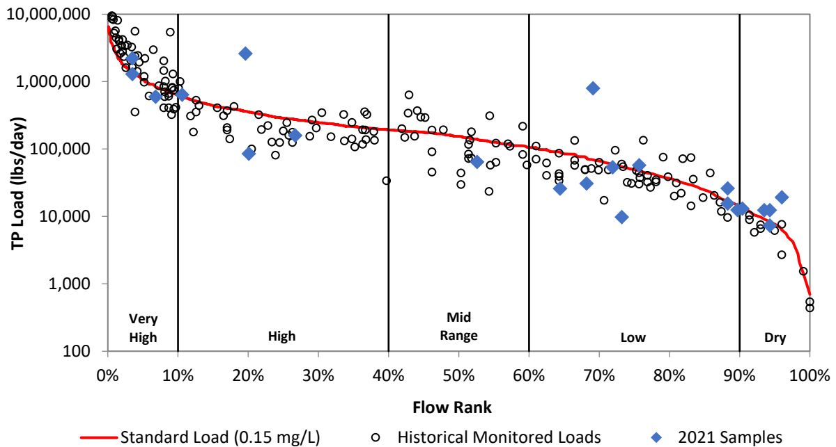
Figure 27a. Load duration curve for total phosphorus at VR24.
