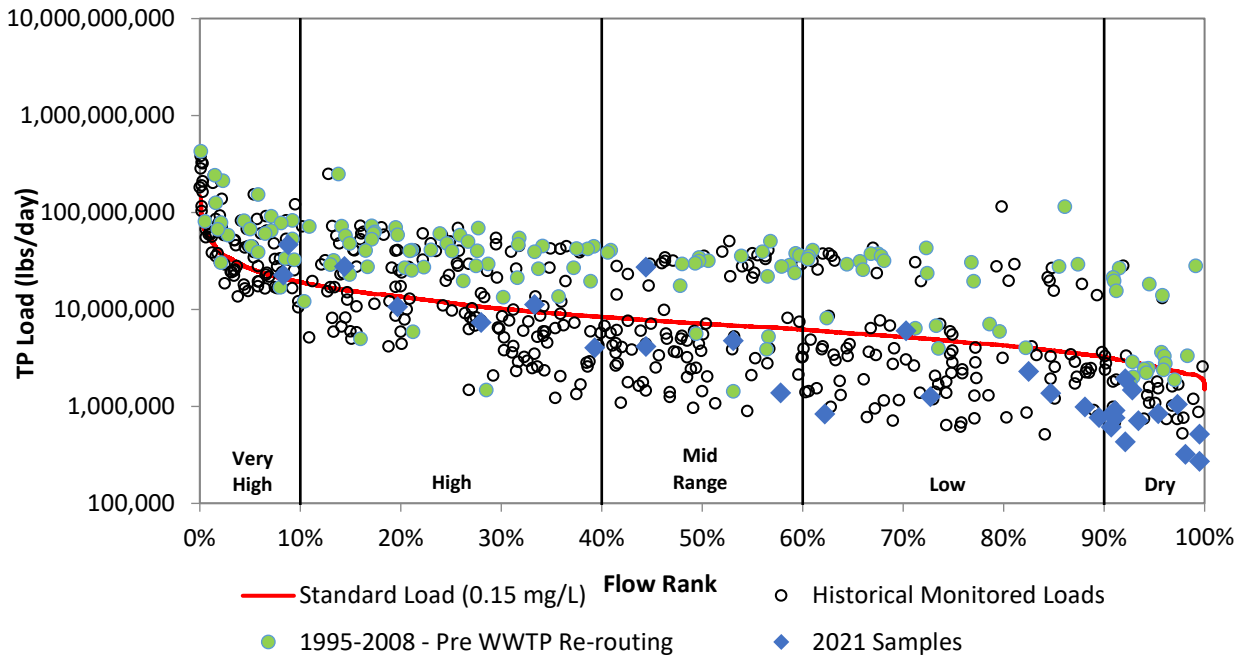
Figure 27i. Load duration curve for total phosphorus at VR0020.
