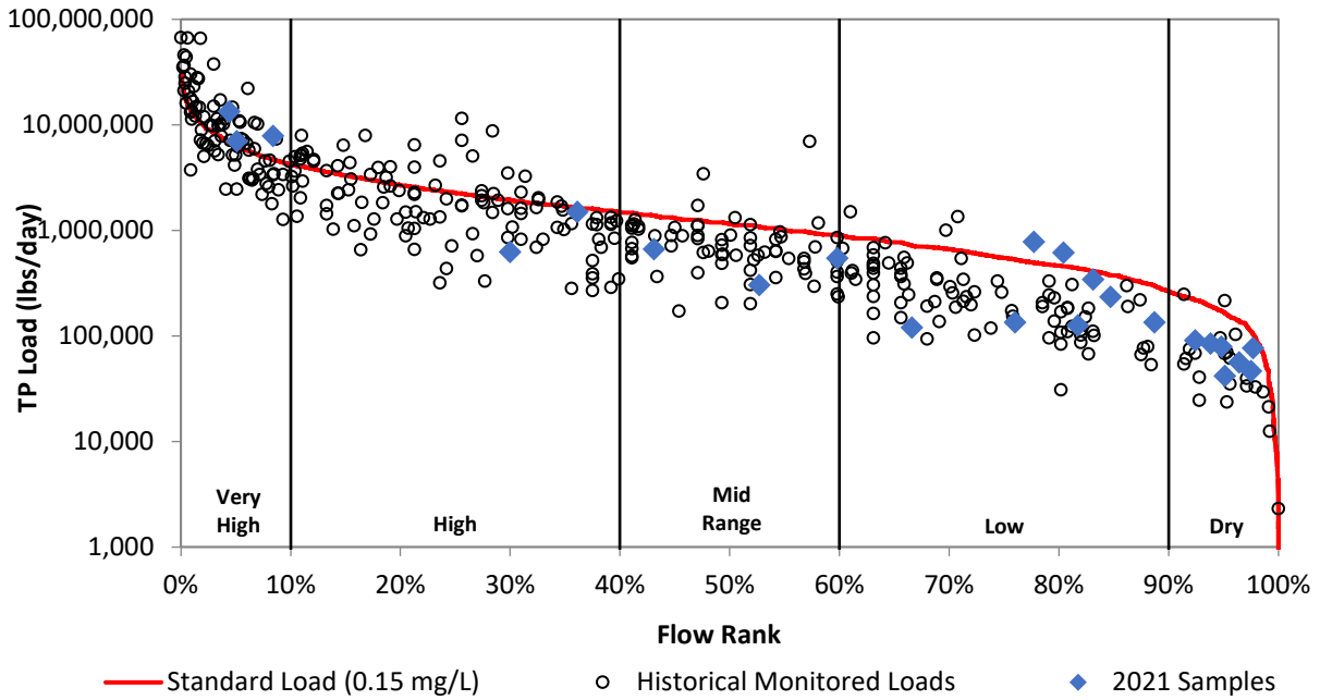
Figure 27c. Load duration curve for total phosphorus at VR804.
