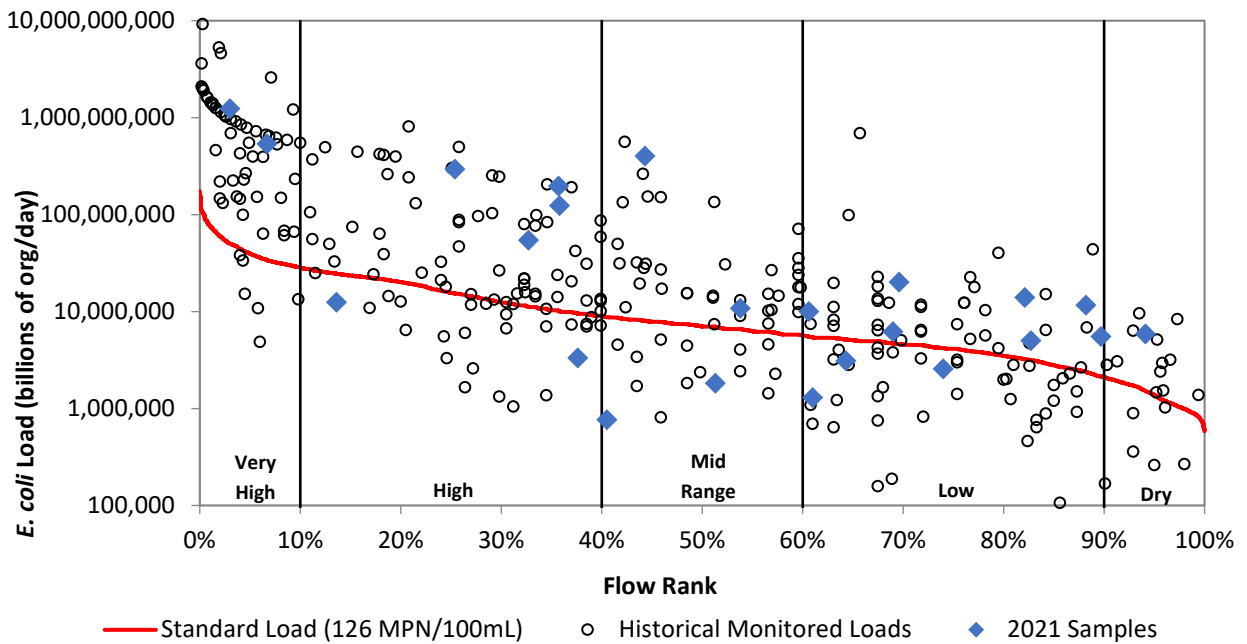
Figure 25f. Load duration curve for E. coli at NC801.
