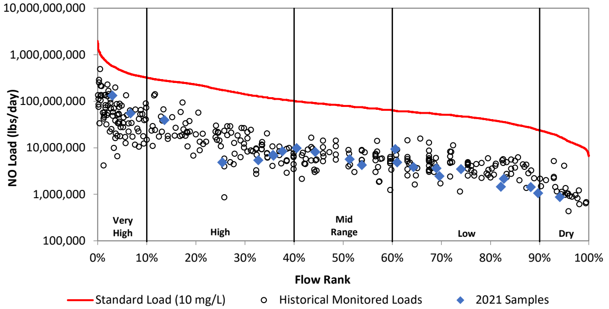
Figure 26f. Load duration curve for nitrate at NC801.
