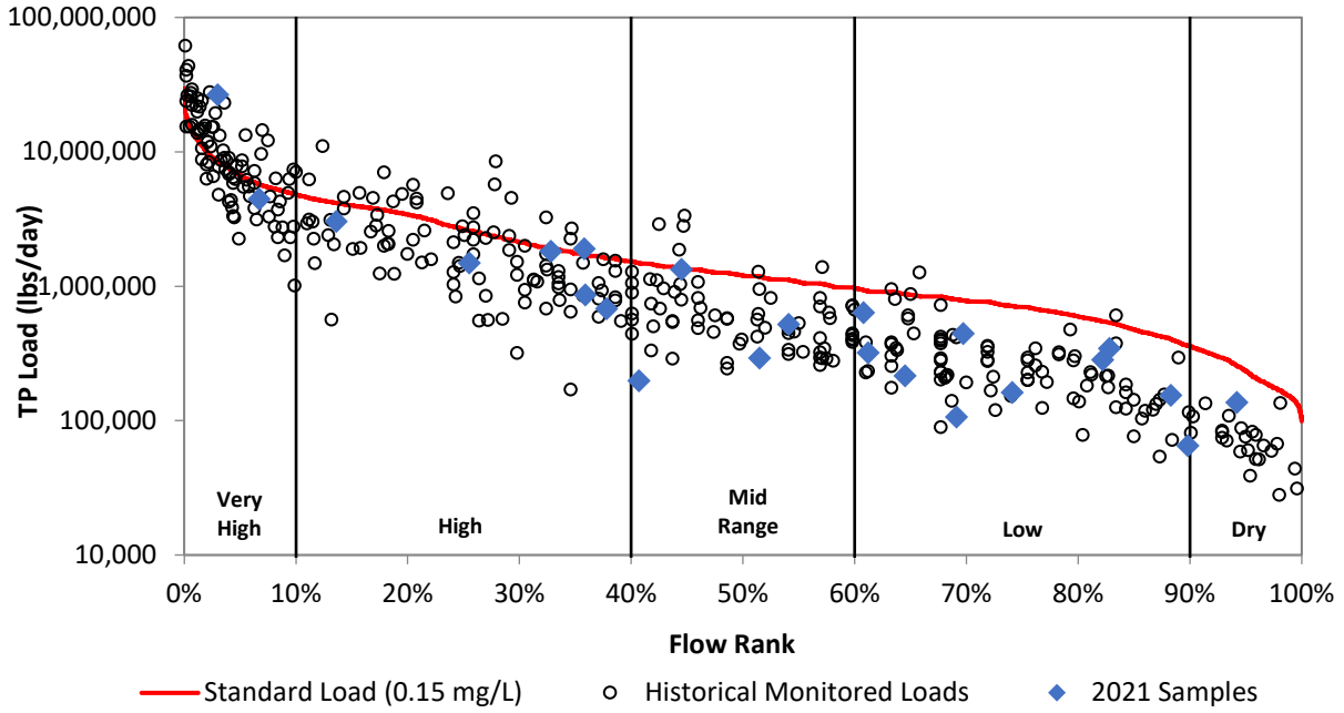
Figure 27f. Load duration curve for total phosphorus at NC801.
