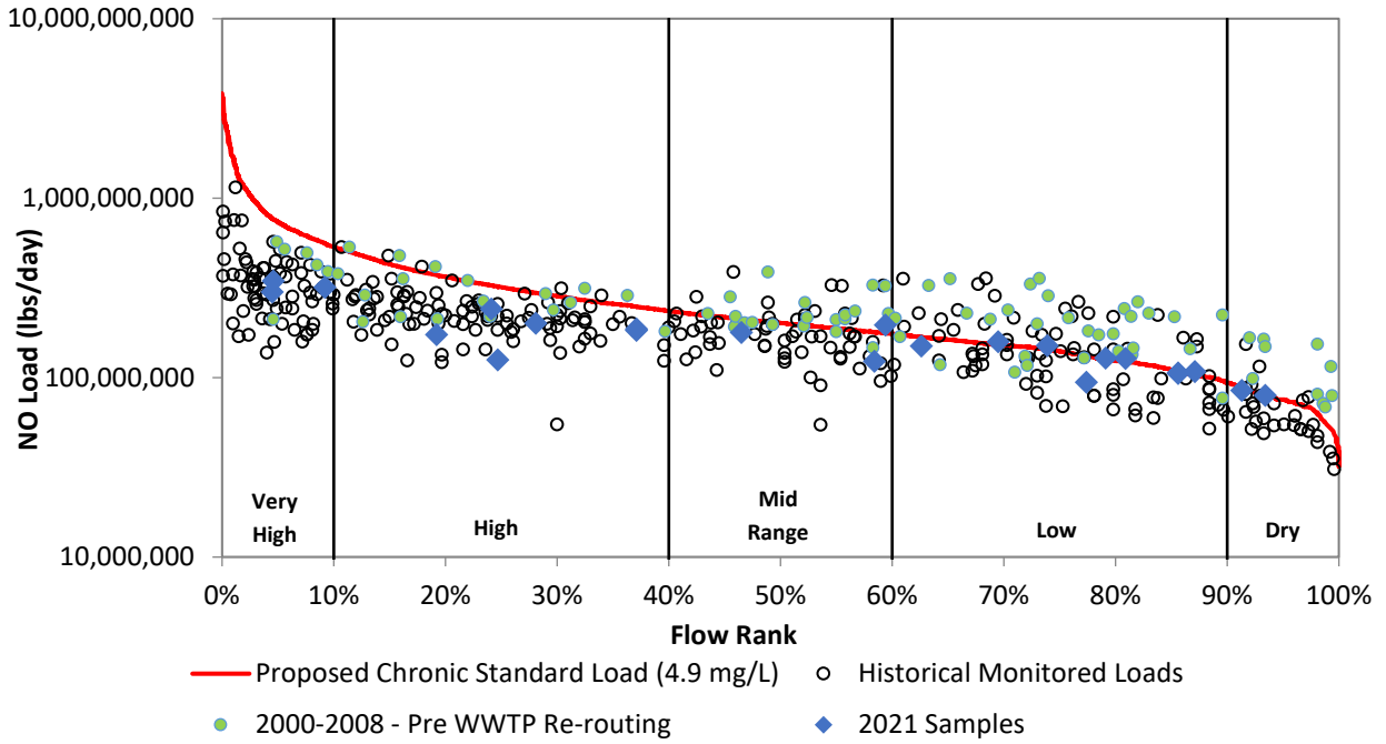
Figure 26h. Load duration curve for nitrate at VR803.
