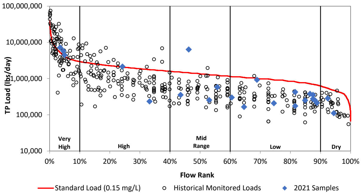
Figure 27g. Load duration curve for total phosphorus at SB802.
