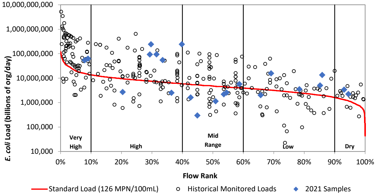
Figure 25e. Load duration curve for E. coli at NC808.
