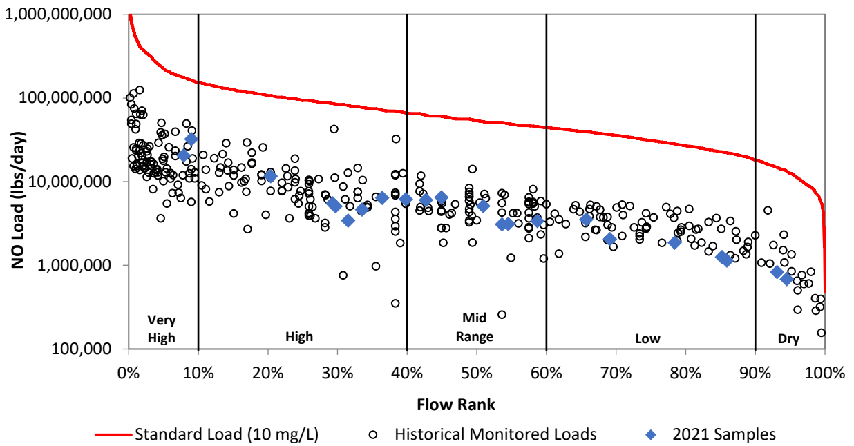
Figure 26e. Load duration curve for nitrate at NC808.
