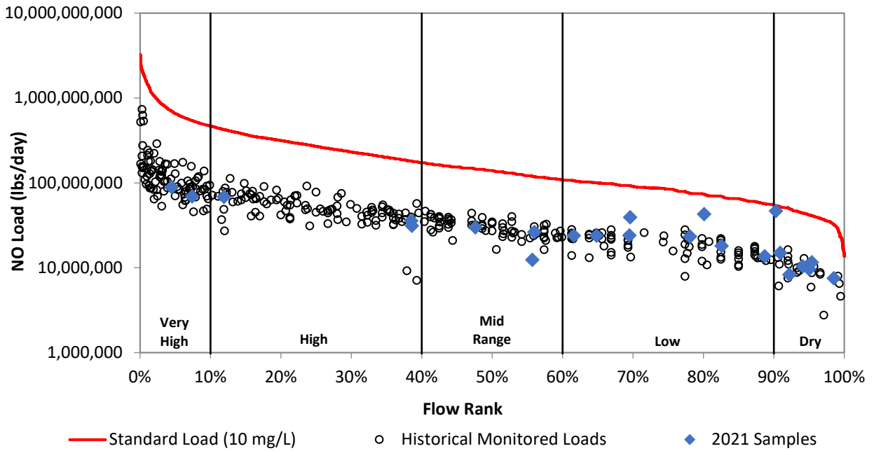
Figure 26d. Load duration curve for nitrate at VR807.
