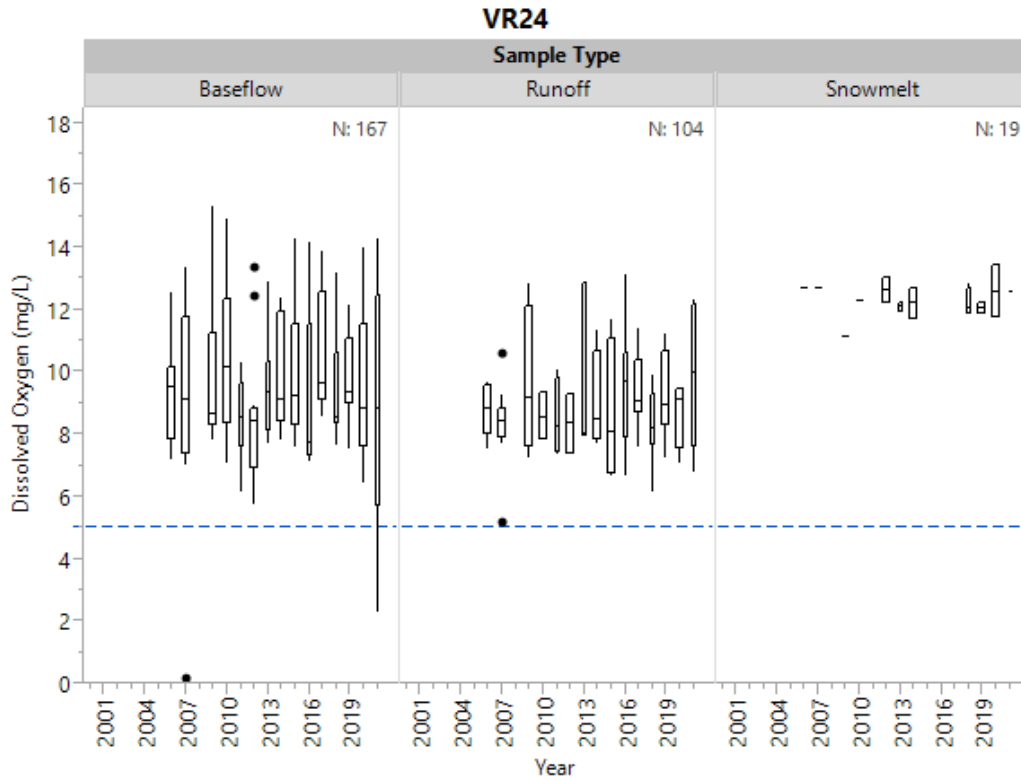
Figure 10a. Historical dissolved oxygen by sample type at VR24.
