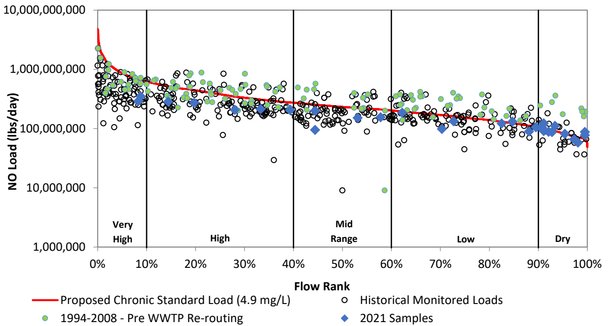
Figure 26i. Load duration curve for nitrate at VR0020.
