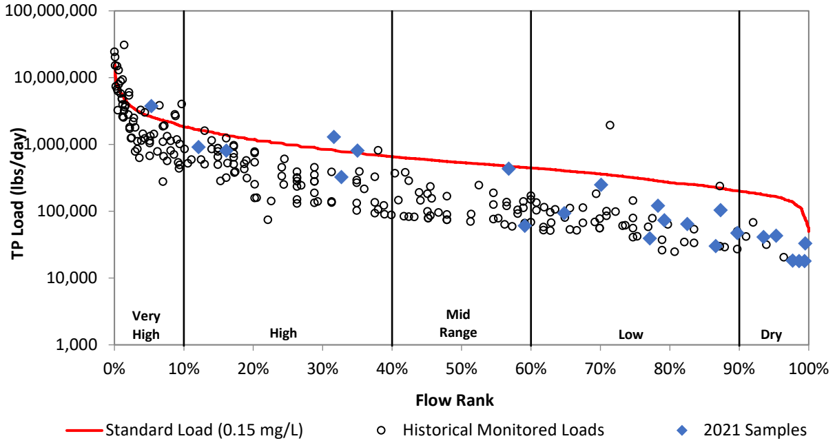
Figure 27b. Load duration curve for total phosphorus at SC806.
