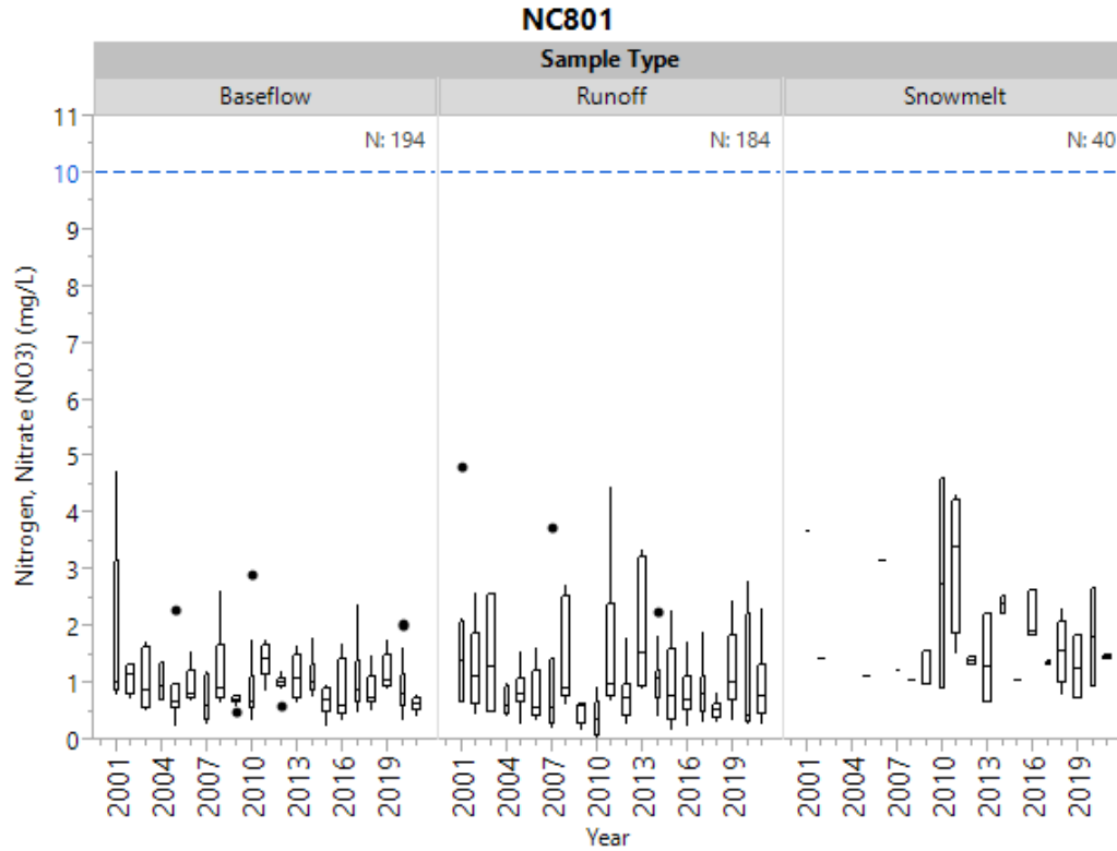
Figure 16f. Historical nitrate by sample type for NC801.
