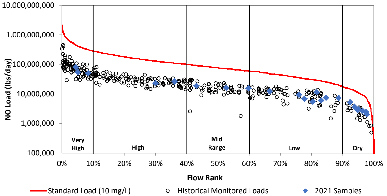
Figure 26c. Load duration curve for nitrate at VR804.
