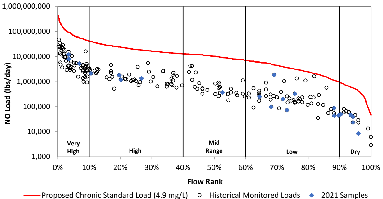
Figure 26a. Load duration curve for nitrate at VR24.
