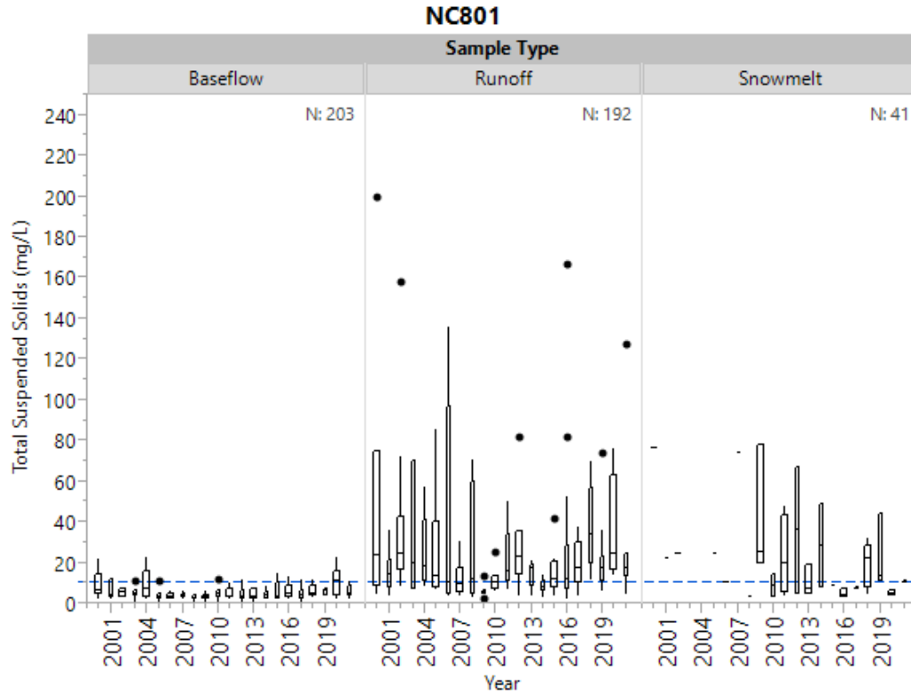
Figure 22f. Historical total suspended solids by sample type at NC801.
