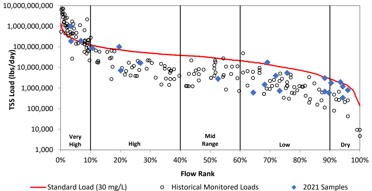
Figure 28a. Load duration curve for total suspended solids at VR24.
